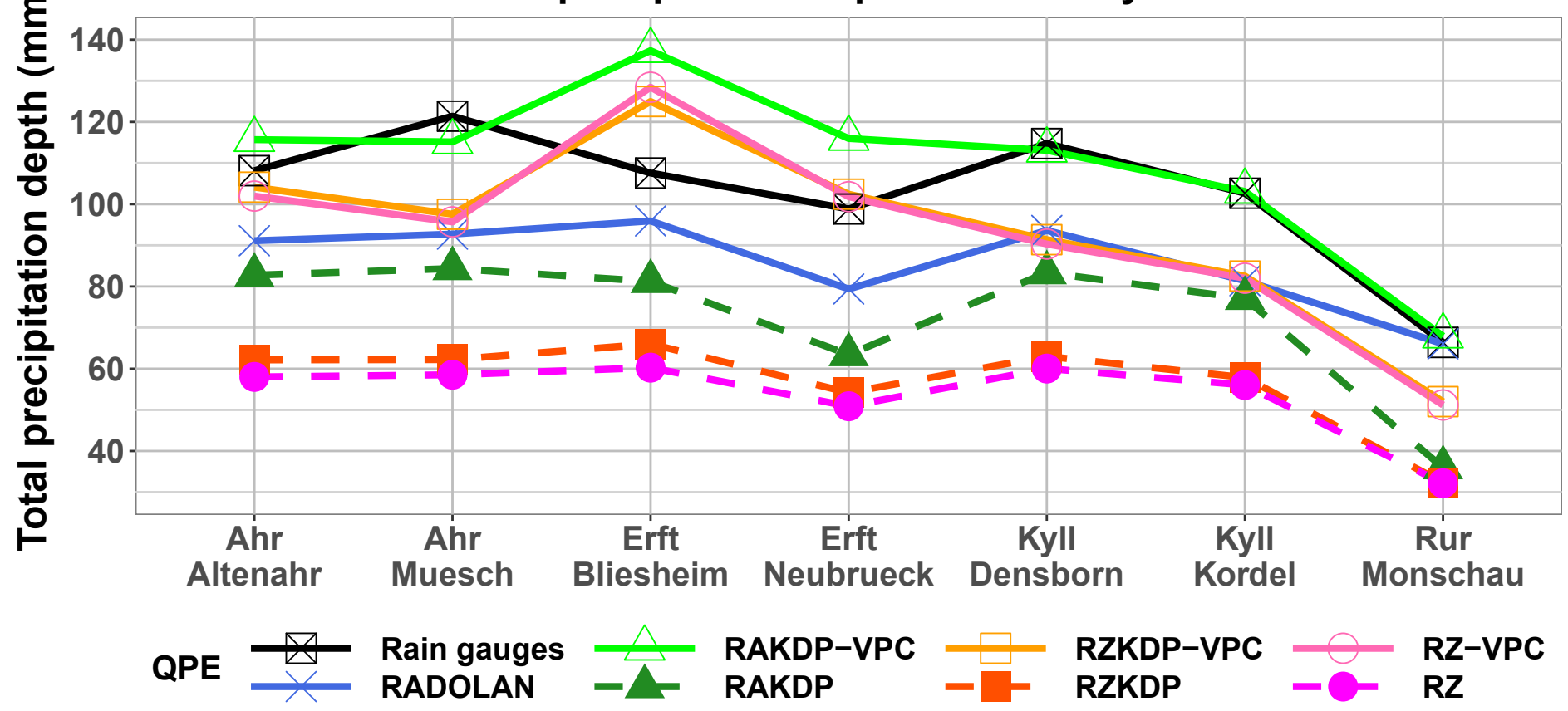
Total precipitation depths on 14 July 2021
