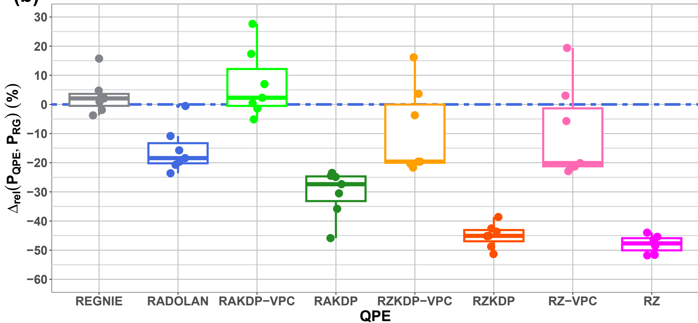
(b) Relative error w.r.t rain gauges
