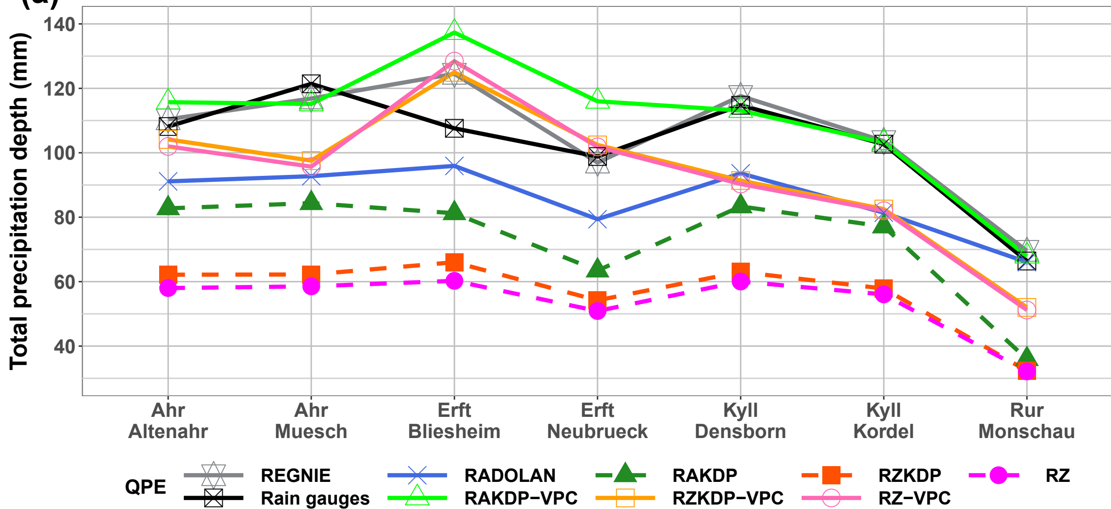
(a) Total precipitation depths on 14 July 2021
