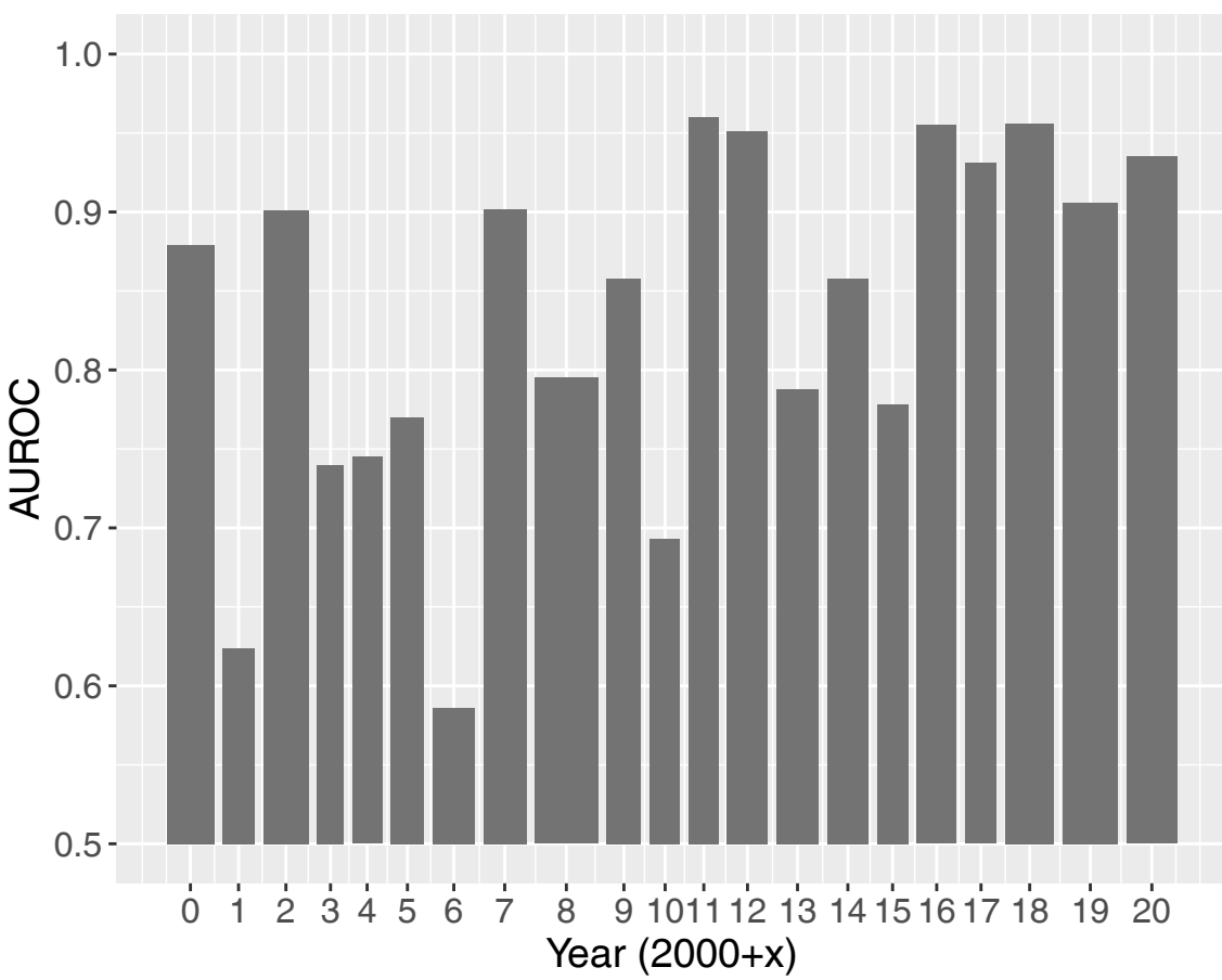
(a) Leave-one-year-out (mAUROC: 0.83)
