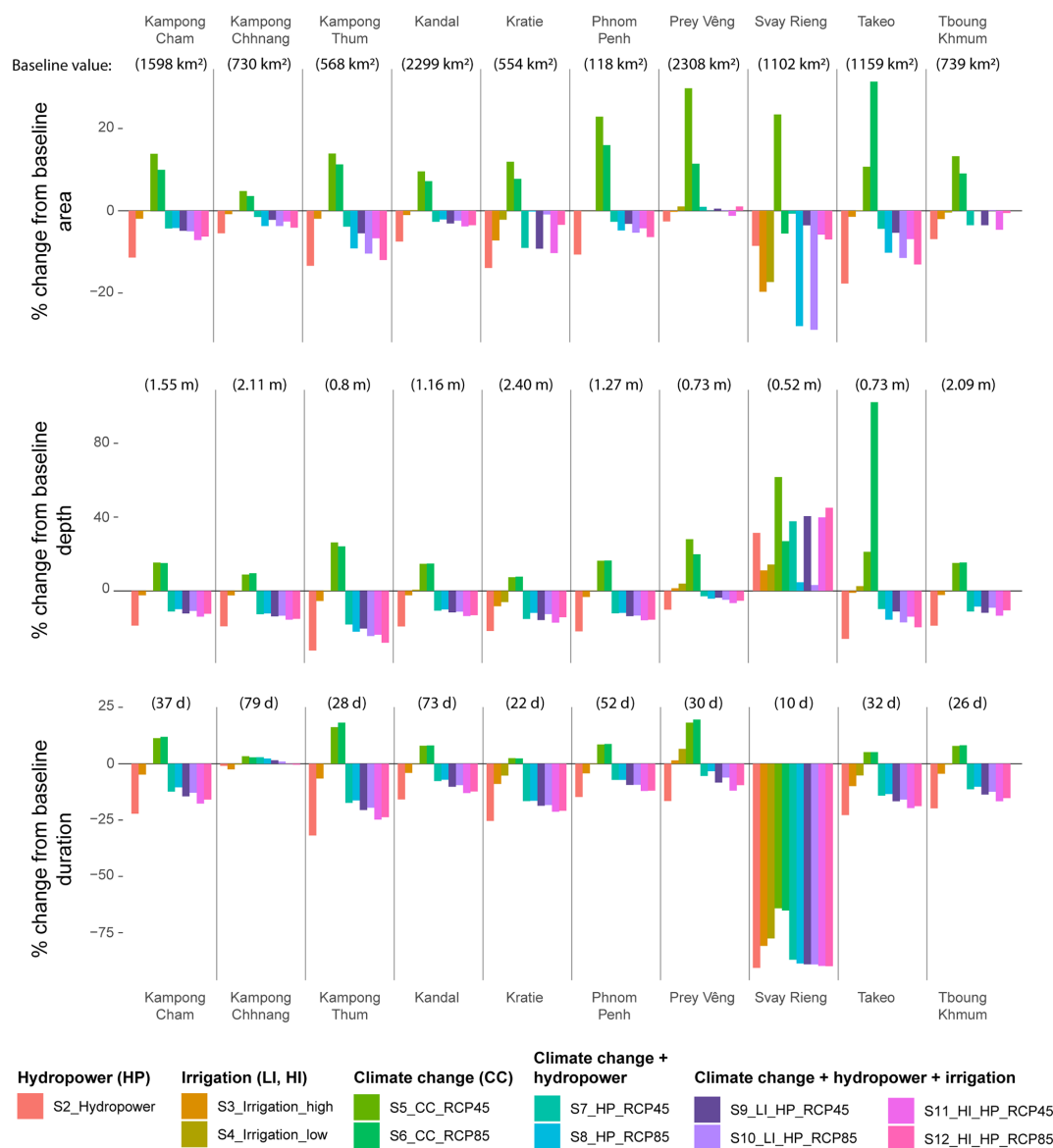
Figure 7. Changes in annual mean flooded area, flood depth, and flood duration compared to the baseline period (1971–2000) for all scenarios at the provincial level. See province location in Fig. 1.
