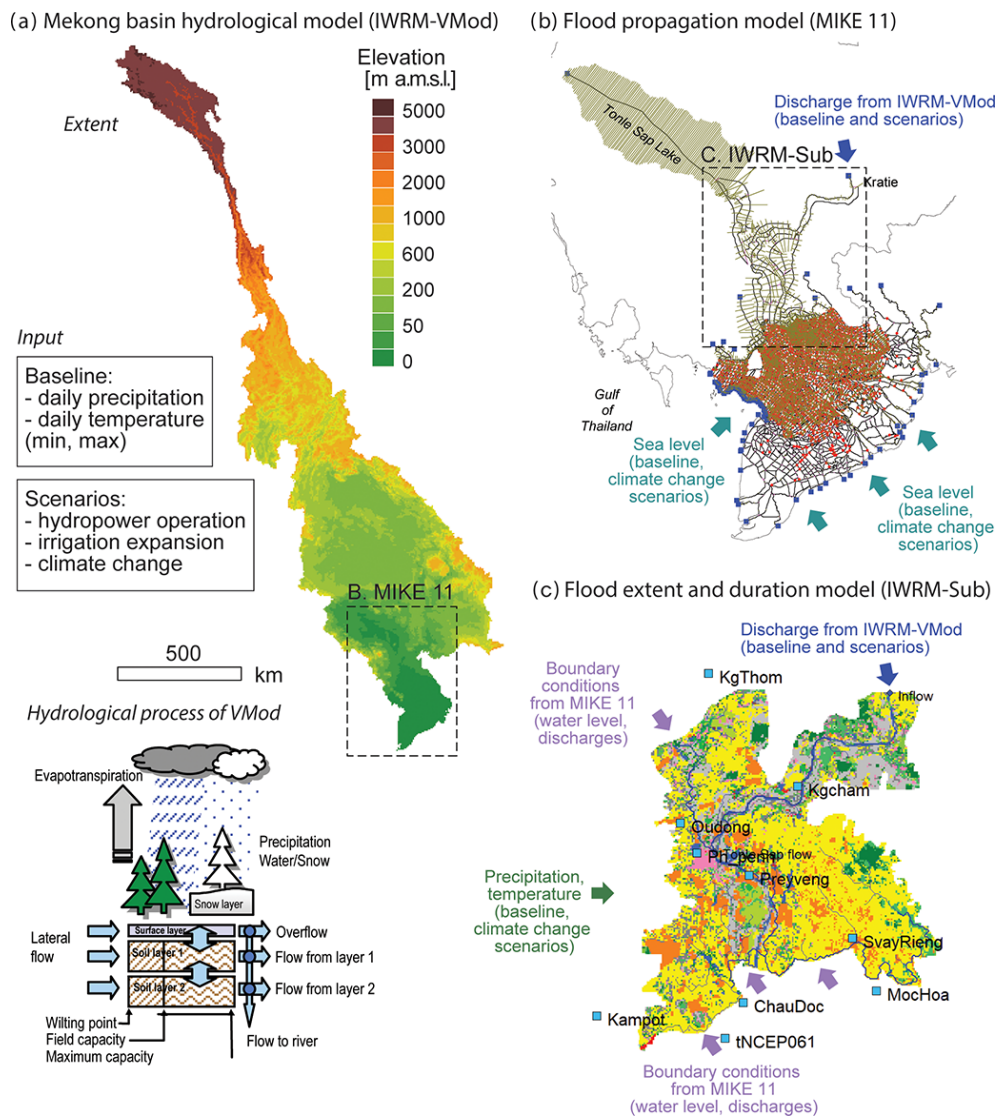
Figure 2. Schematic illustration of the modelling setup. (a) Mekong basin hydrological model IWRM-VMod models the hydrology of the entire Mekong basin with 5 km \times 5 km resolution (Hoang et al., 2019). (b) Flood propagation model MIKE 11 models the hydrodynamics of the entire Mekong floodplain using the discharges from IWRM-VMod and sea level in South China Sea as boundary conditions (Triet et al., 2017). (c) Flood extent and duration model IWRM-Sub is a detailed 2D floodplain model using the output from two other models as an input.
