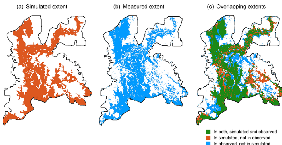
Figure 3. Comparison of maximum flood extent resulting from the model and measured from satellite images.
