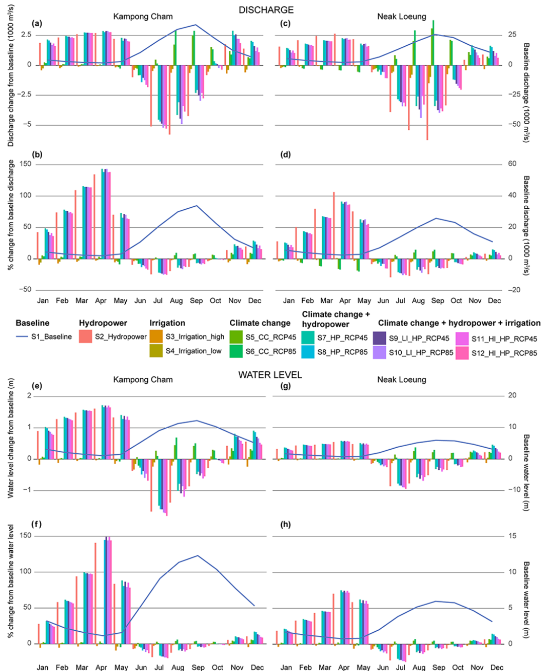
Figure 4. Changes in monthly water discharge and water level at Kampong Cham (left-hand side) and Neak Loeung (right-hand side); the blue line indicates the baseline monthly discharge and water level, and the colour bar charts indicate both the magnitude (a, c, e, g) and the percentage (b, d, f, h) change under different scenarios in comparison with the baseline (1971–2000). (See location of stations in Fig. 1.)
