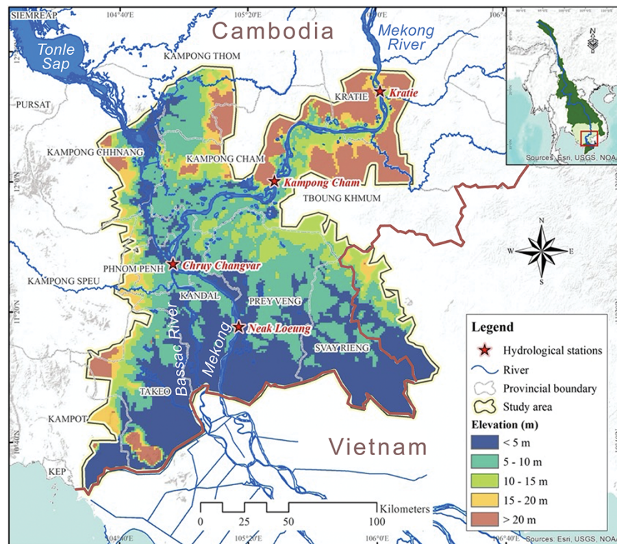
Figure 1. Map of the study area, the Cambodian Mekong floodplain. Elevation of 90 m grid cell was extracted from the SRTM database, and river lines were obtained from the MRC database.
