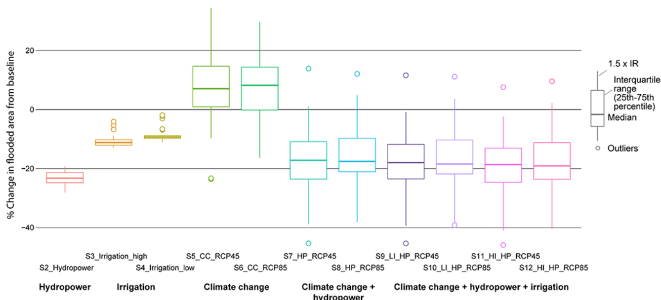
Figure 5. Changes in total flooded area compared to the baseline period 1971–2000; the graph shows the range of changes due to interannual variation (box and whiskers), the median change (horizontal line), and outliers that were exceptional years (circles).
