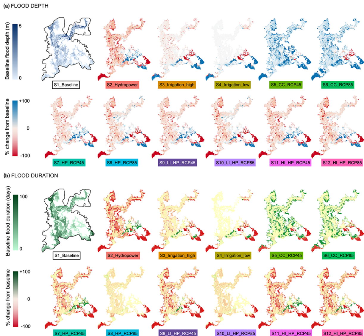
Figure 6. Spatial distribution of changes in flood depth and duration. (a) Flood depth; (b) flood duration. Results are shown over the baseline period 1971–2000 and all scenarios (see description in Table 2).
