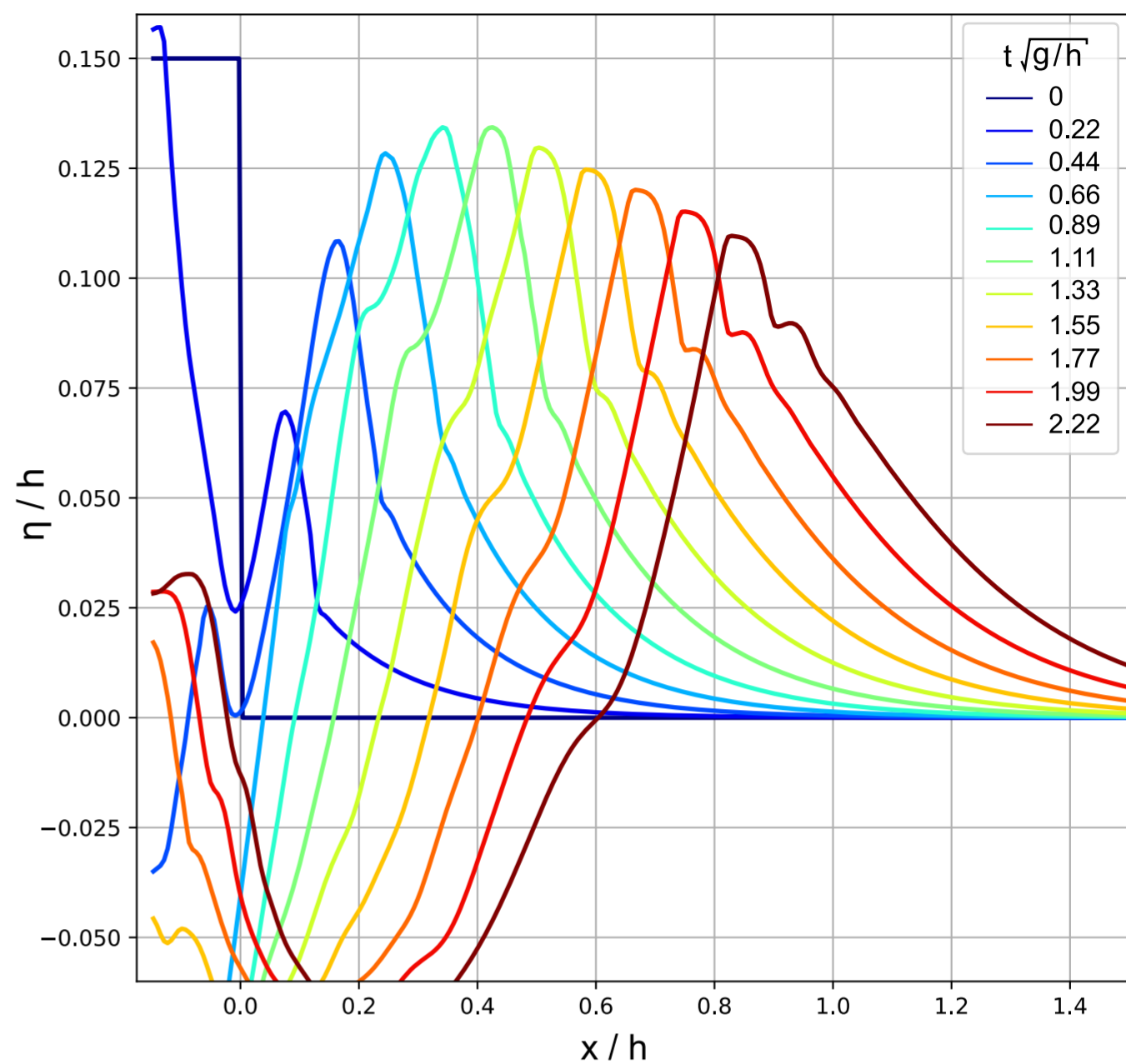
(b) Serre-Green-Naghdi
