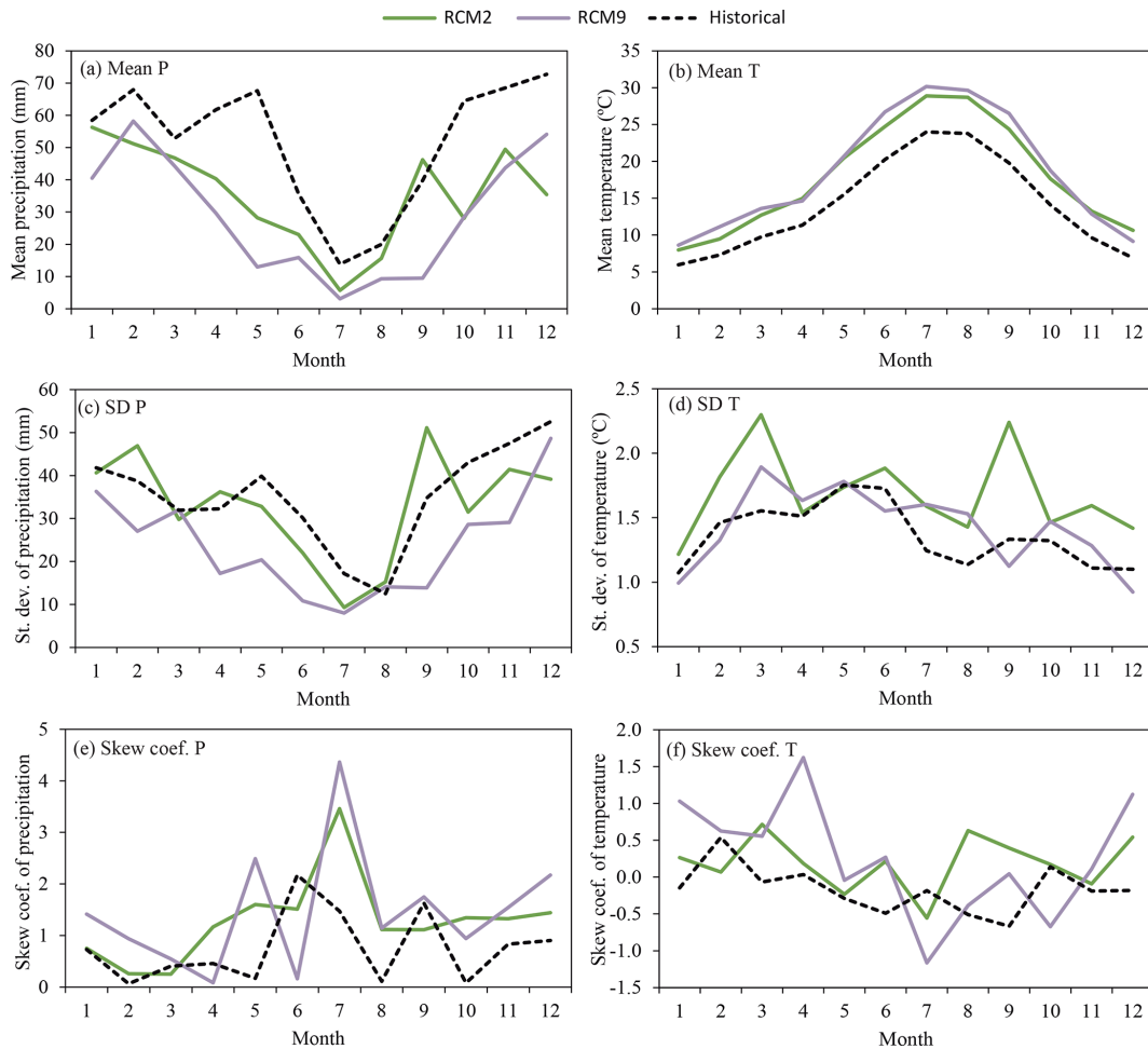
Figure 10. Monthly mean, standard deviation and skew coefficient within the mean year of the historical period (1972–2002) and future horizon (2071–2100) series (RCM2 and 9) for precipitation (a, c, e) and temperature (b, d, f).
