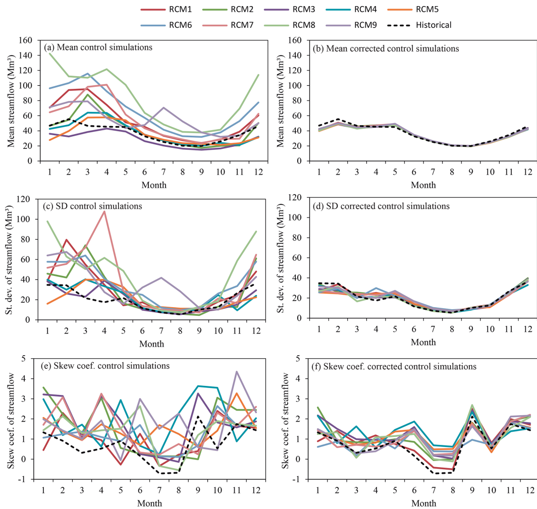
Figure 7. Monthly mean, standard deviation and skew coefficient of streamflow within the mean year of the period (1972–2001) for the historical and control simulation series (a, c, e) and historical and corrected control simulation series (b, d, f).
