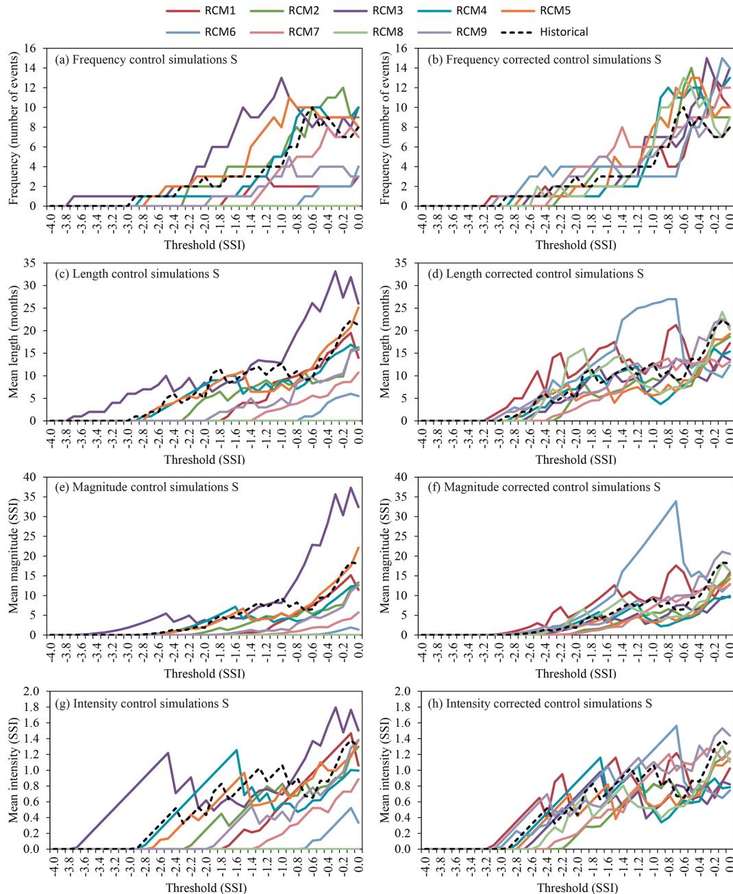
Figure 9. Drought statistics (frequency, length, magnitude and intensity) of the period (1972–2001) for the historical and control simulation series (a, c, e, g) and the historical and corrected control simulation series (b, d, f, h) for streamflow (hydrological droughts).
