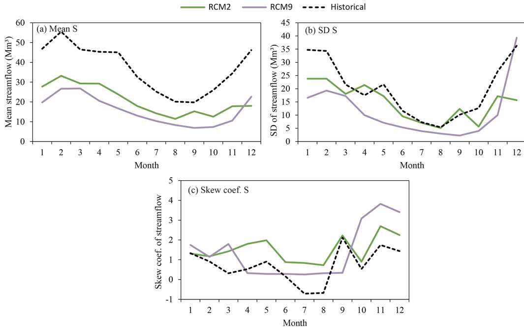
Figure 11. Monthly mean (a), standard deviation (b) and skew coefficient (c) within the mean year of the historical period (1972–2002) and future horizon (2071–2100) series (RCM2 and RCM9) for streamflow.
