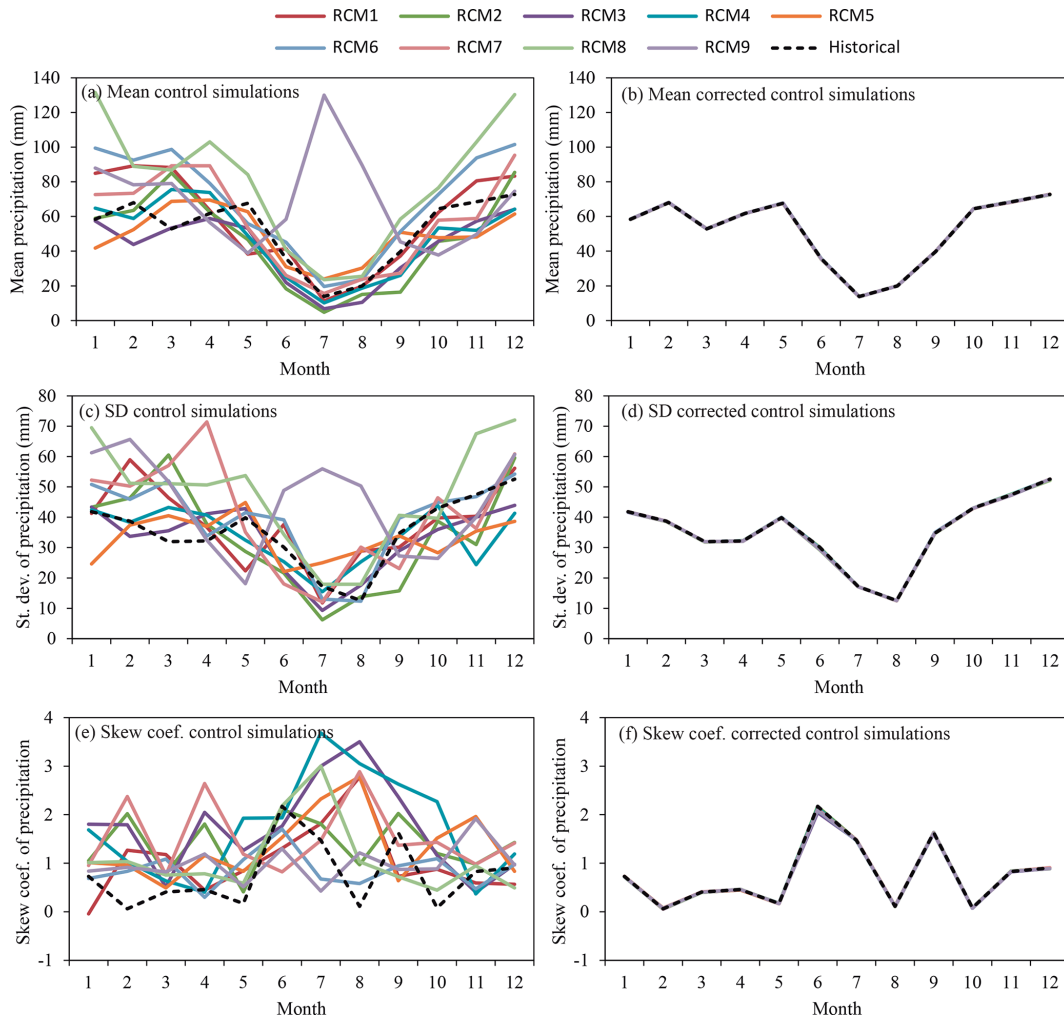
Figure 4. Monthly mean, standard deviation and skew coefficient of precipitation within the mean year of the period (1972–2001) for the historical and control simulation series ( a, c, e ) and historical and corrected control simulation series ( b, d, f ).
