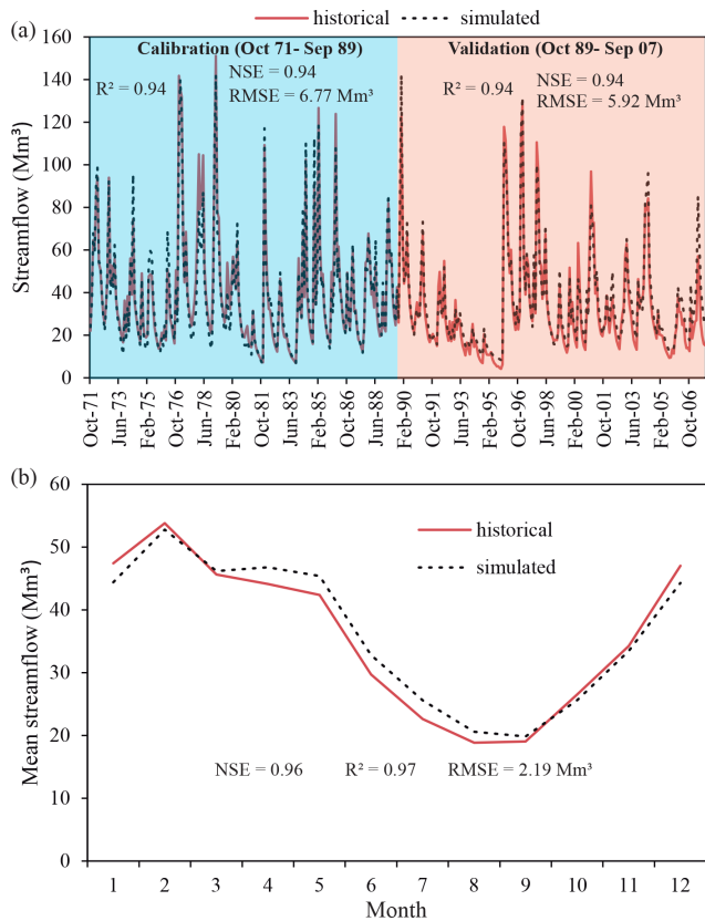
Figure 3. Historical and simulated monthly streamflow series in the Cenajo basin for the calibration period (October 1971 to September 1989) and the validation period (October 1989 to September 2007) (a) and mean monthly values within the mean year of the entire period (October 1971 to September 2007) (b).
