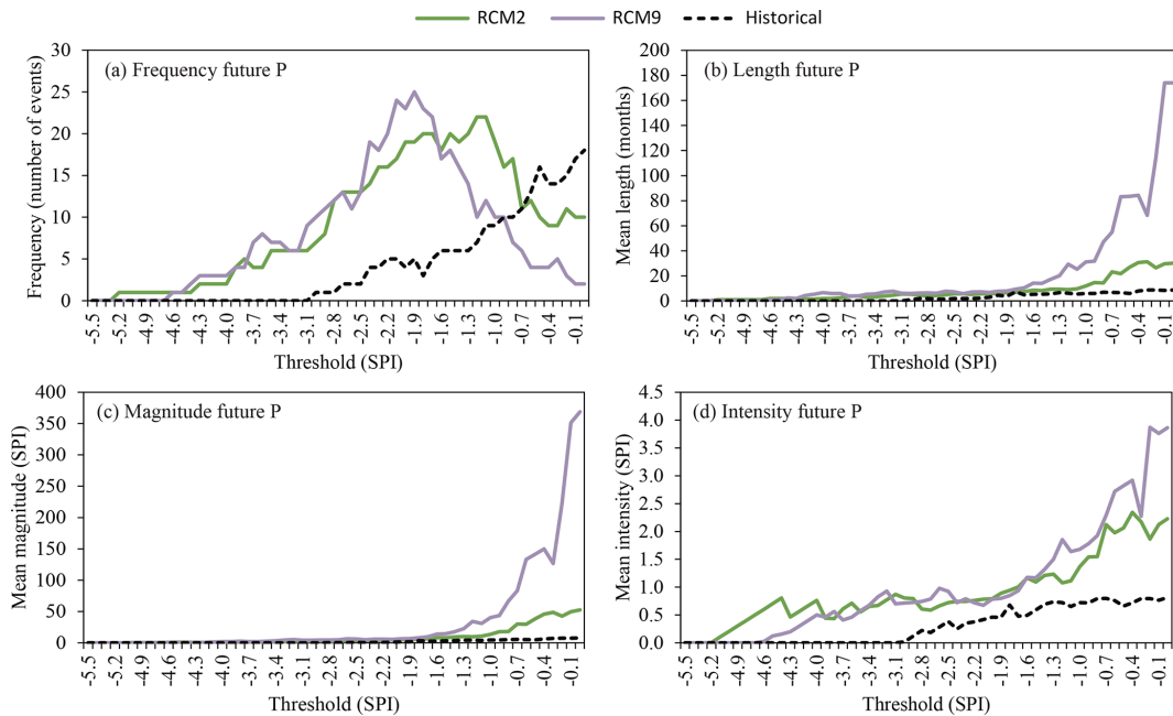
Figure 12. Drought statistics – (a) frequency, (b) length, (c) magnitude, (d) intensity – of the historical period (1972–2002) and future horizon (2071–2100) series (RCM2 and RCM9) for precipitation (meteorological droughts).
