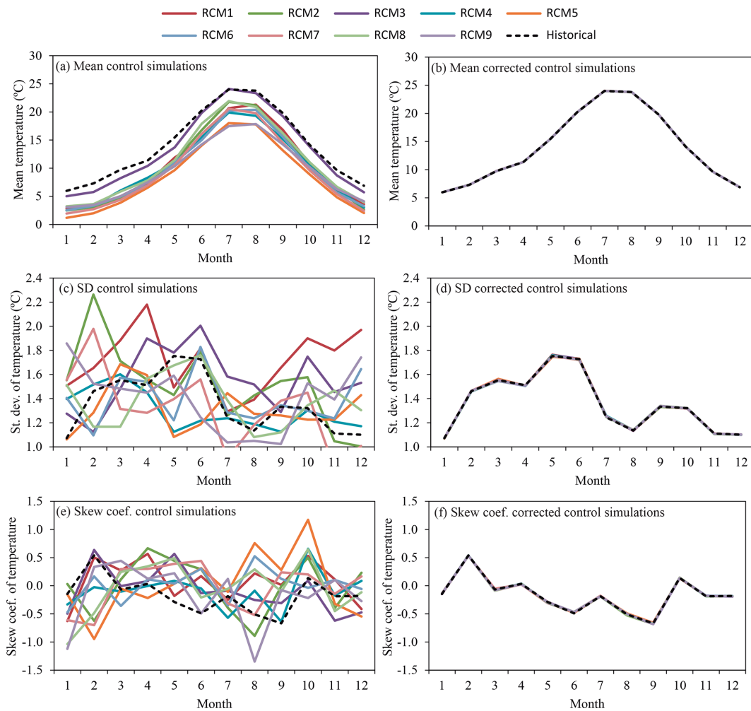
Figure 5. Monthly mean temperature, standard deviation, and skew coefficient of temperature within the mean year of the period (1972–2001) for the historical and control simulation series ( a, c, e ) and historical and corrected control simulation series ( b, d, f ).
