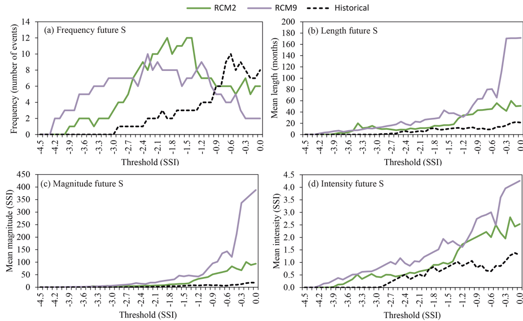
Figure 13. Drought statistics – (a) frequency, (b) length, (c) magnitude, (d) intensity – of the historical period (1972–2002) and future horizon (2071–2100) series (RCM2 and 9) for streamflow (hydrological droughts).
