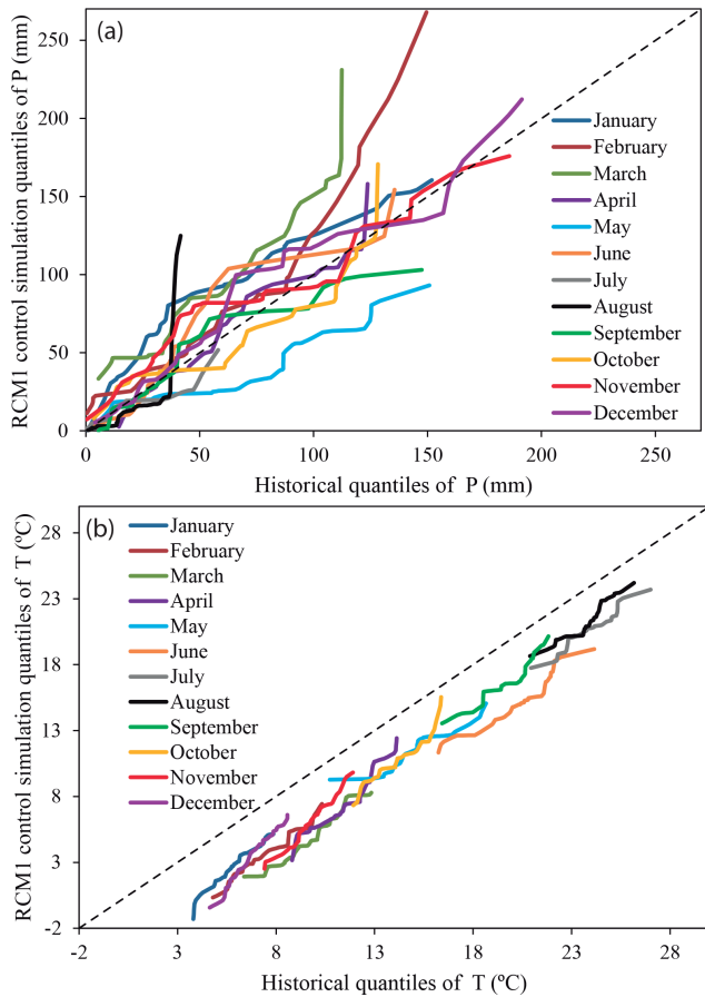
Figure 6. Precipitation (a) and temperature (b) quantiles of the observed and control series of the RCM1 simulations for each month of the year in the reference period (1972–2001).
