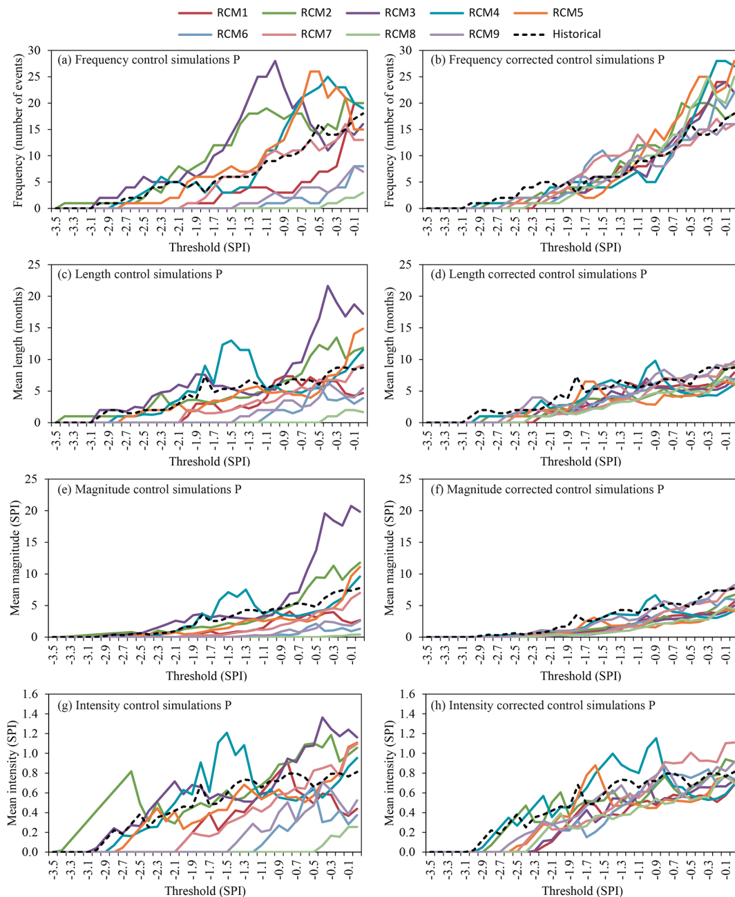
Figure 8. Drought statistics (frequency, length, magnitude and intensity) of the period (1972–2001) for the historical and control simulation series (a, c, e, g) and historical and corrected control simulation series (b, d, f, h) for precipitation (meteorological droughts).
