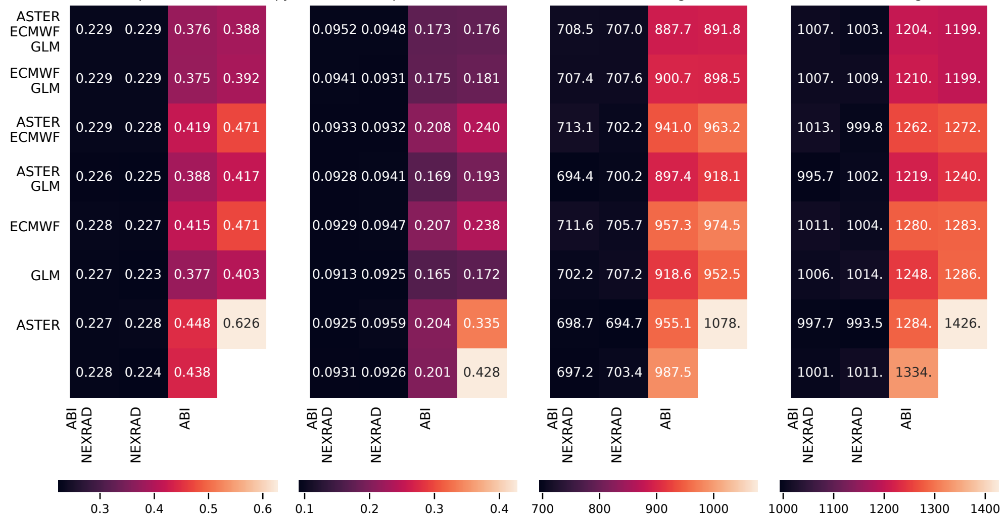
(a) 45 dBZ ET presence cross-entropy
