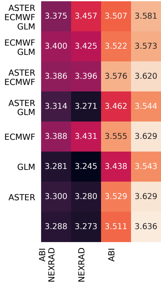
(a) Maximum reflectivity MAE
