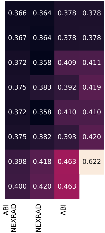
(c) Lightning occ. cross-entropy
