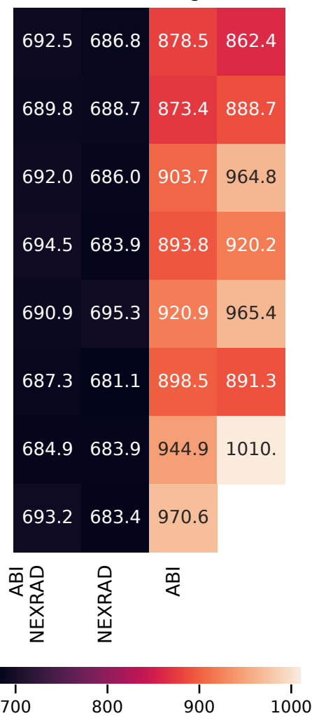
(c) 45 dBZ ET height MAE
