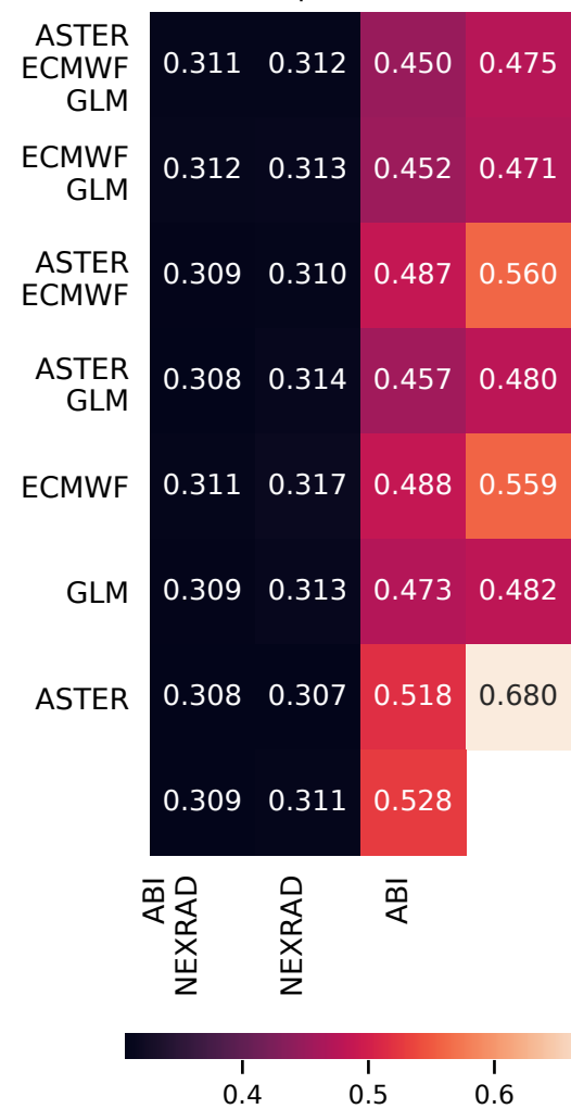
(a) 45 dBZ ET presence cross-entropy
