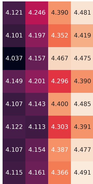
(b) Maximum reflectivity RMSE
