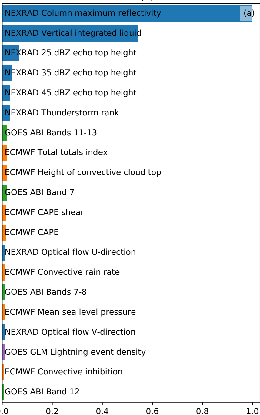
45 dBZ echo top presence
