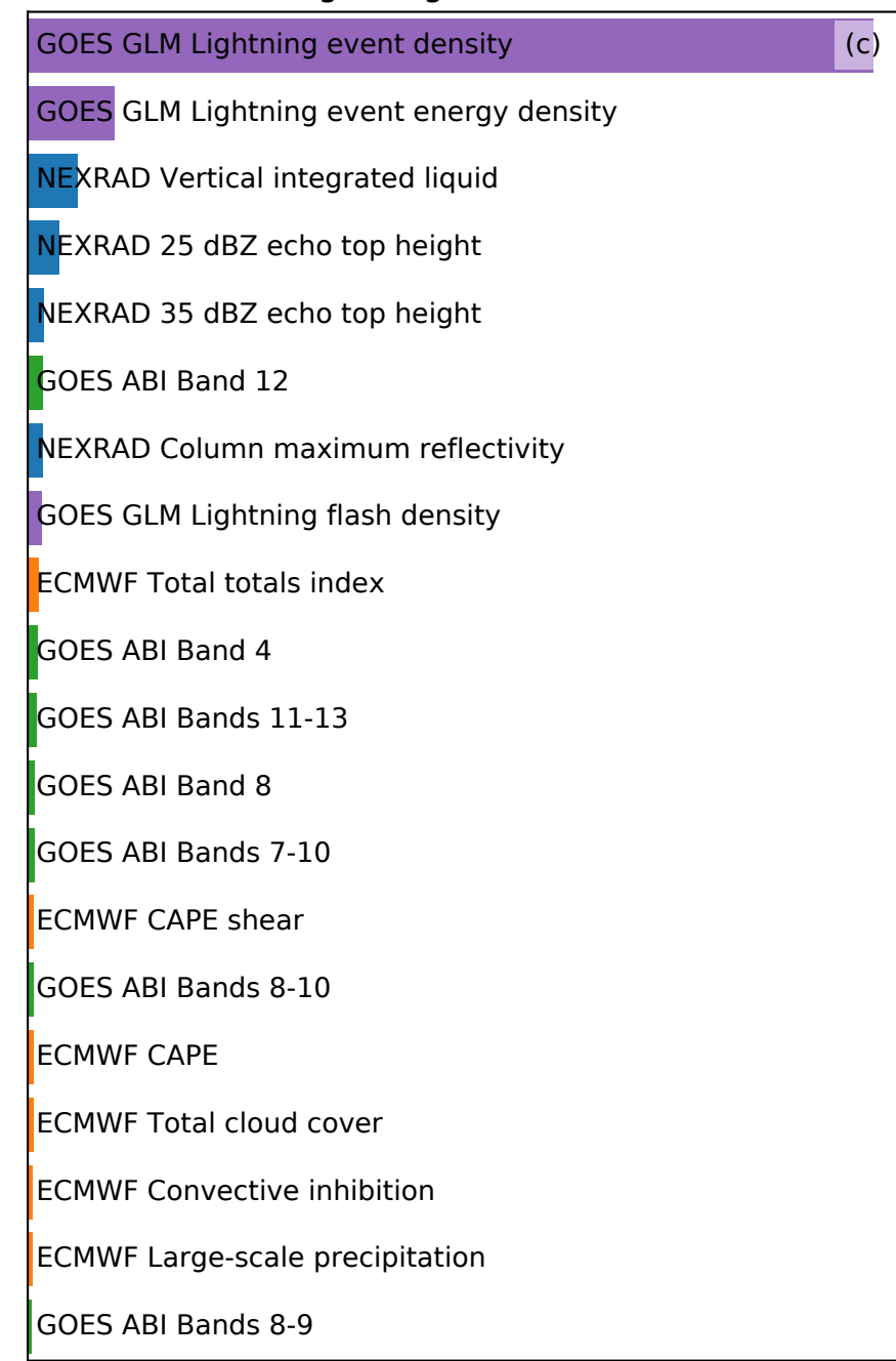
Lightning occurrence
