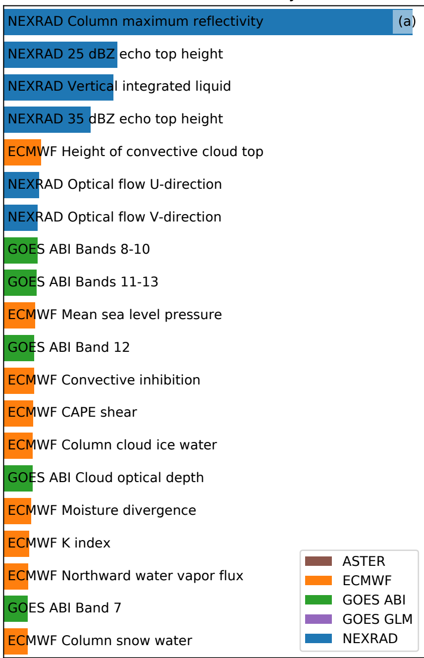
Maximum reflectivity
