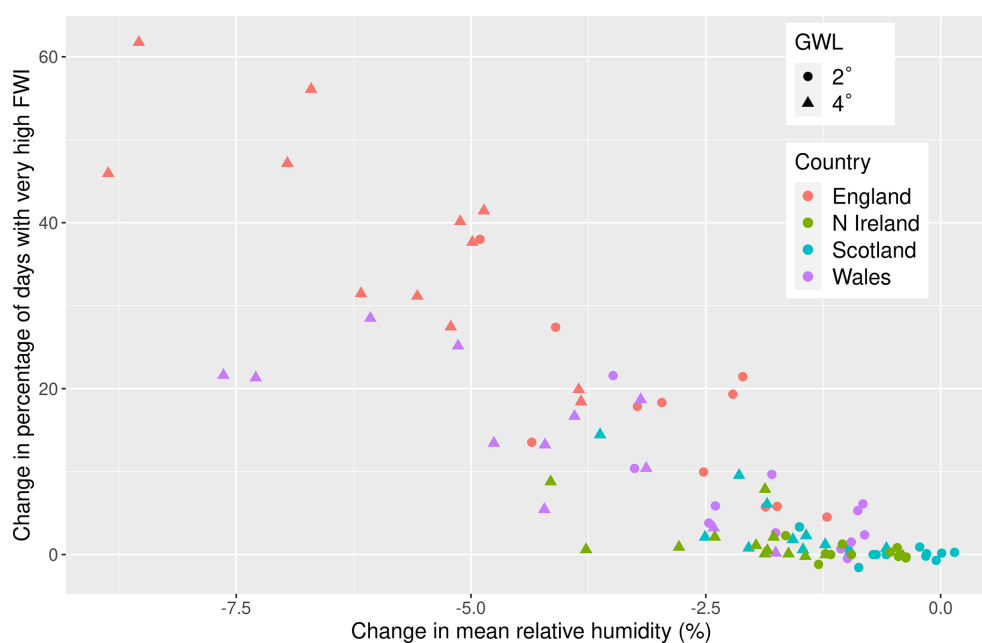
Figure 11. Scatter plot of change in the percentage of summer days with very high FWI against change in mean relative humidity (%), by country and ensemble member. Changes are from 1981–2010 to the 2 and 4 °C global warming levels.
