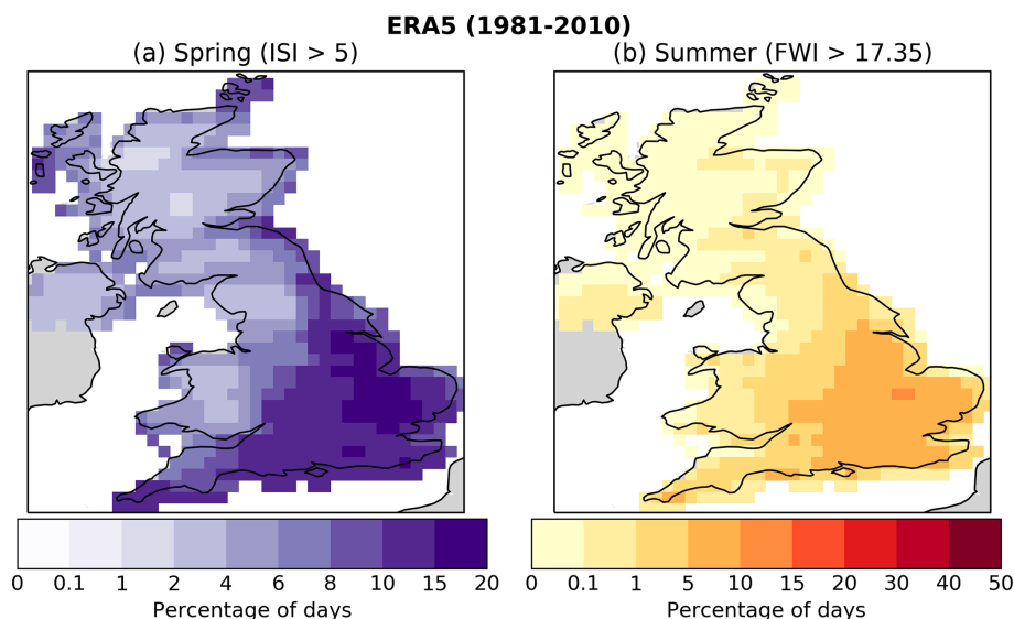
Figure 8. Percentage of days with dangerous fire weather for (a) spring (ISI > 5 ; at least high) and (b) summer (FWI > 17.35 ; at least very high). Based on the ERA5 reanalysis data for the 1981–2010 period.
