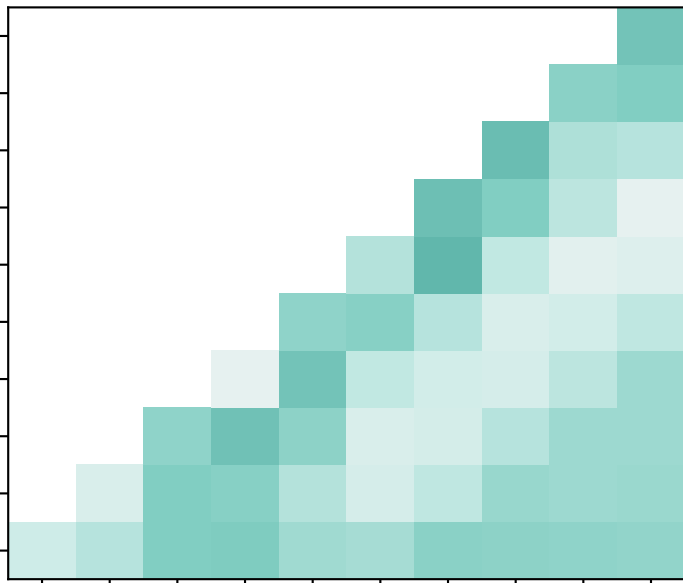
(a) High Storm Activity
