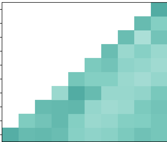
(e) Moderate Storm Activity
