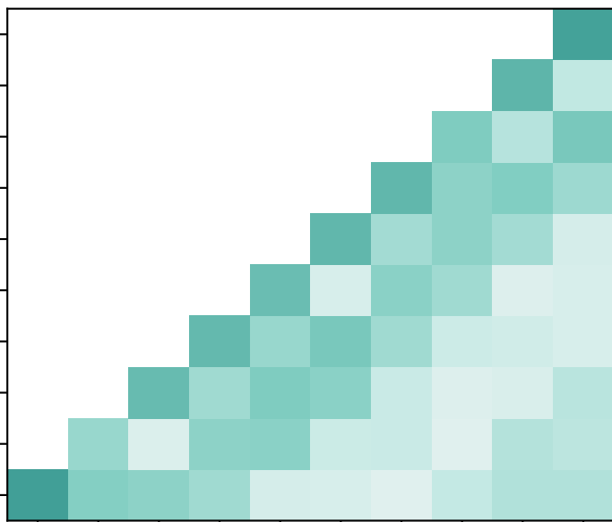
(c) Low Storm Activity
