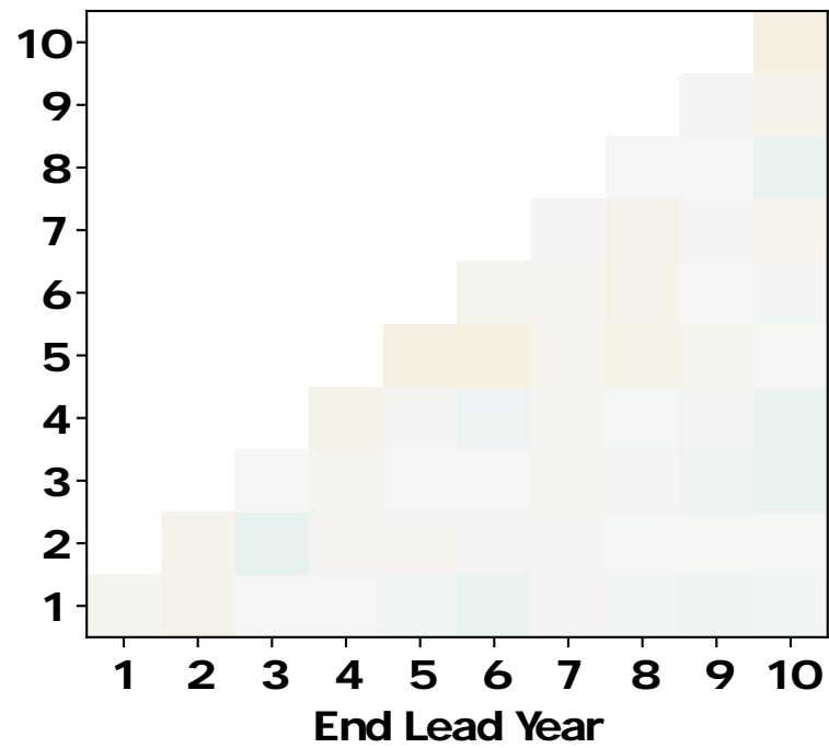
(f) Moderate Storm Activity
