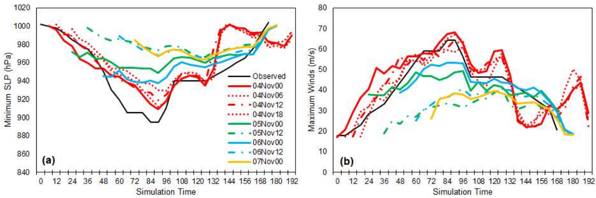
Supplementary Figure 6: Time series of (a) minimum sea level pressure in hPa and (b) maximum winds in ms-1 for the sensitivity experiments with different initial times, including the simulated tracks (c) for the experiments initialized at 04 Nov 00UTC, 05 Nov 00UTC, 06 Nov 00UTC, and 07 Nov 00UTC.
