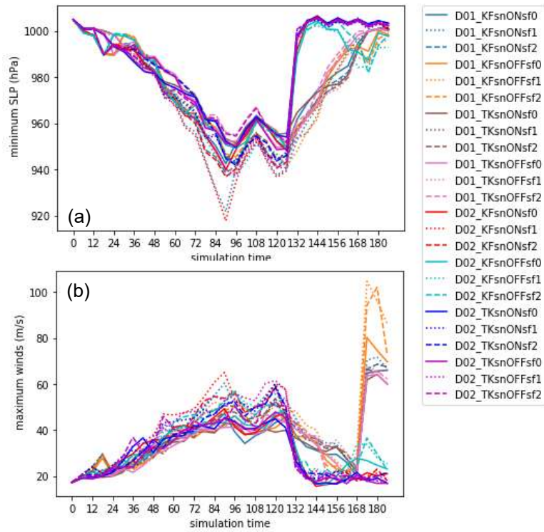
55 Supplementary Figure 8: Time series of simulated 6-hourly (a) minimum sea level pressure in hPa and (b) maximum winds in ms-1 for the sensitivity experiments from 04 Nov 00 UTC (t=0) to 11 Nov 18 UTC (t=186) from the mother/outer domain (D01) and child/inner domain (D02) for all sensitivity experiments.
