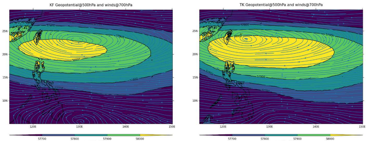
Supplementary Figure 11: Average Geopotential height at 500hPa in geopotential meters (shaded contour lines) and winds (streamlines) at 700hPa averaged over the entire period of the simulation with (a) KF and (b) TK. The 6-hourly WRF output was interpolated to the coarser 6-hourly ERA5 grid using First-order Conservative Remapping through CDO remapcon function. CDO code available at https://code.mpimet.mpg.de/projects/cdo/
