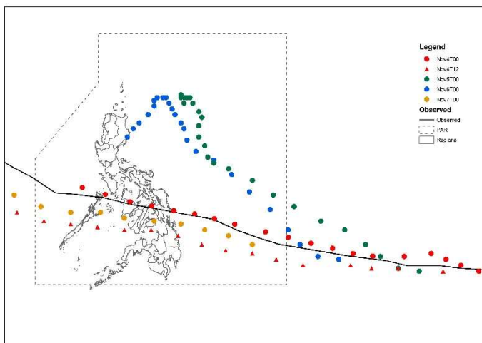
Supplementary Figure 7: Time series of (a) minimum sea level pressure in hPa and (b) maximum winds in ms-1 for the sensitivity experiments with different initial times, including the simulated tracks (c) for the experiments initialized at 04 Nov 00UTC, 05 Nov 00UTC, 06 Nov 00UTC, and 07 Nov 00UTC.
