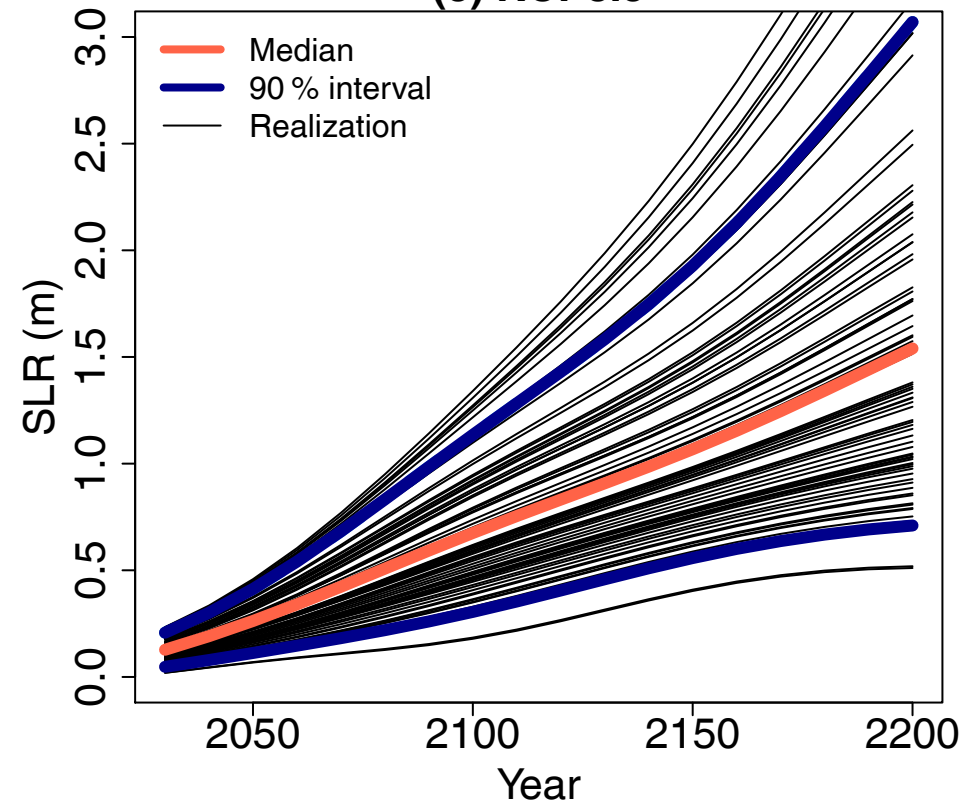
(c) RCP8.5
