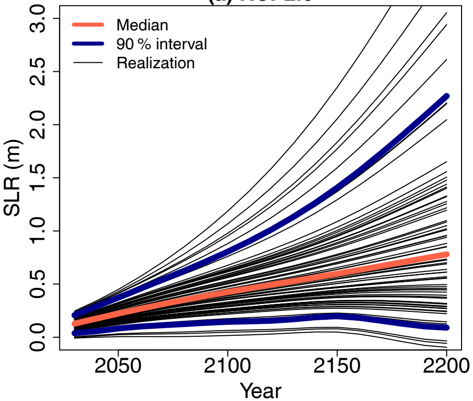
(a) RCP2.6
