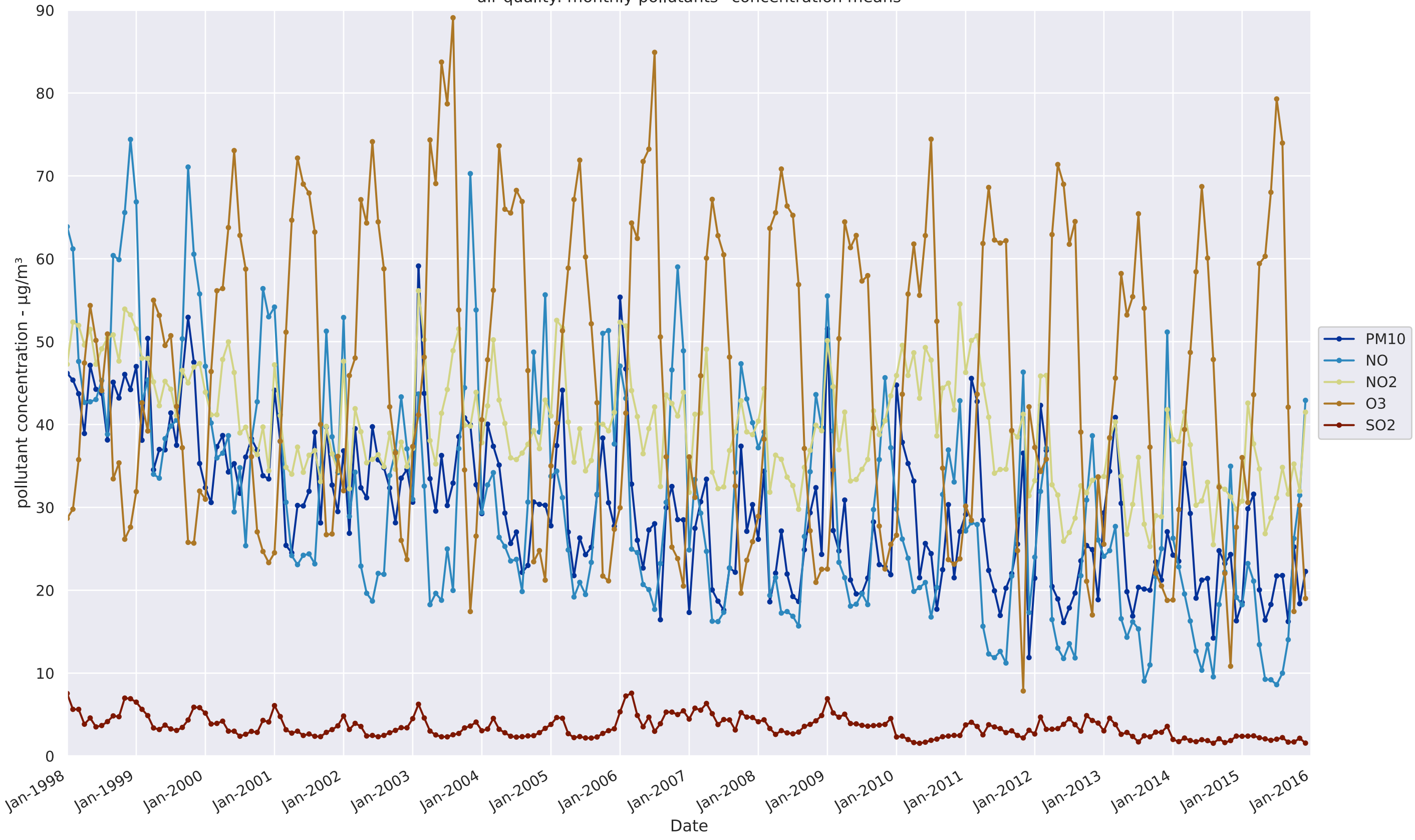
air quality: monthly pollutants' concentration means
