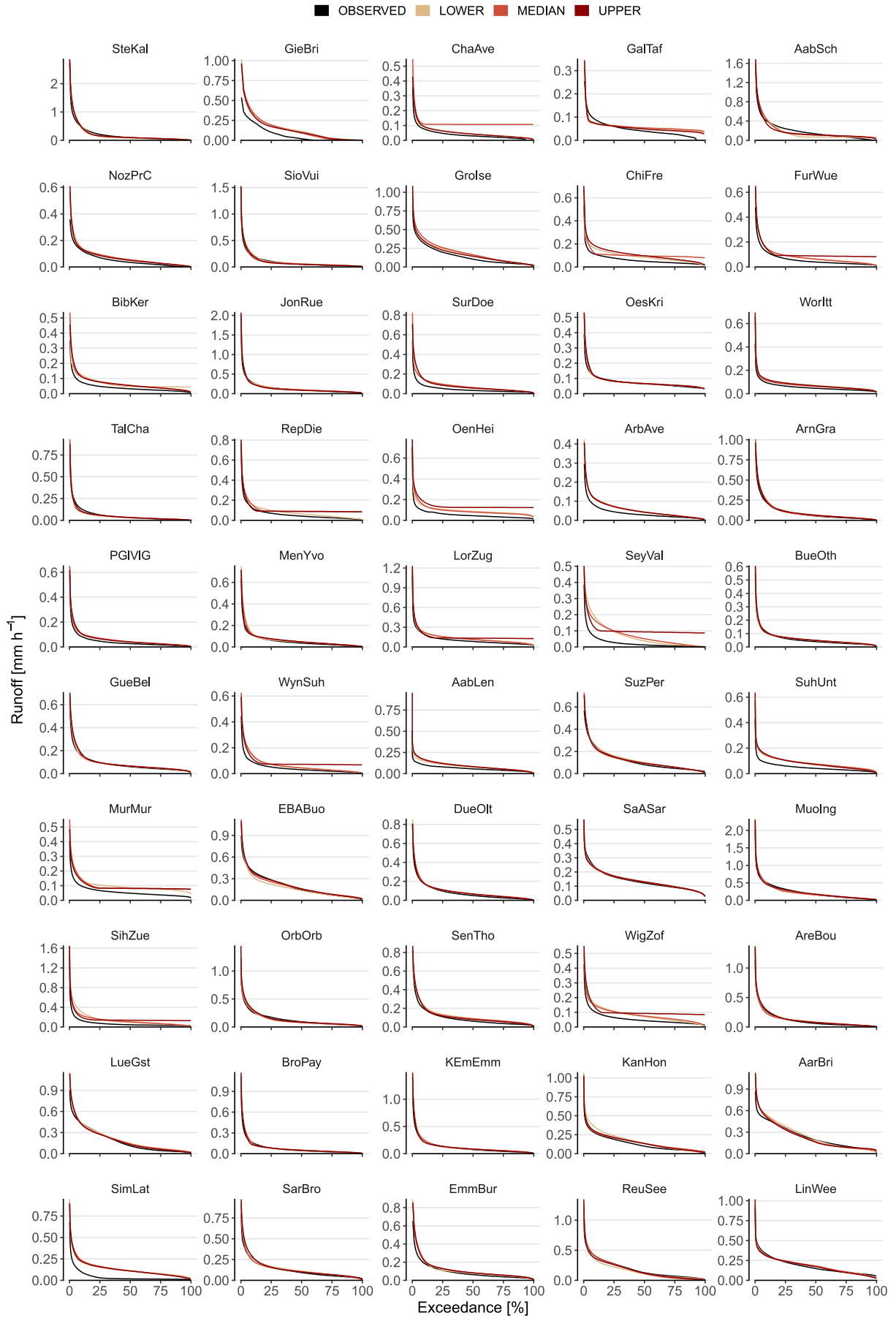
Figure S1. Flow duration curves for 50 gauged sub-catchments simulated with HBV (lower, median and upper representative parameter sets; time period 1930–2014; ordered by increasing catchment area) in comparison to observations (varying time periods, see Table S2).
