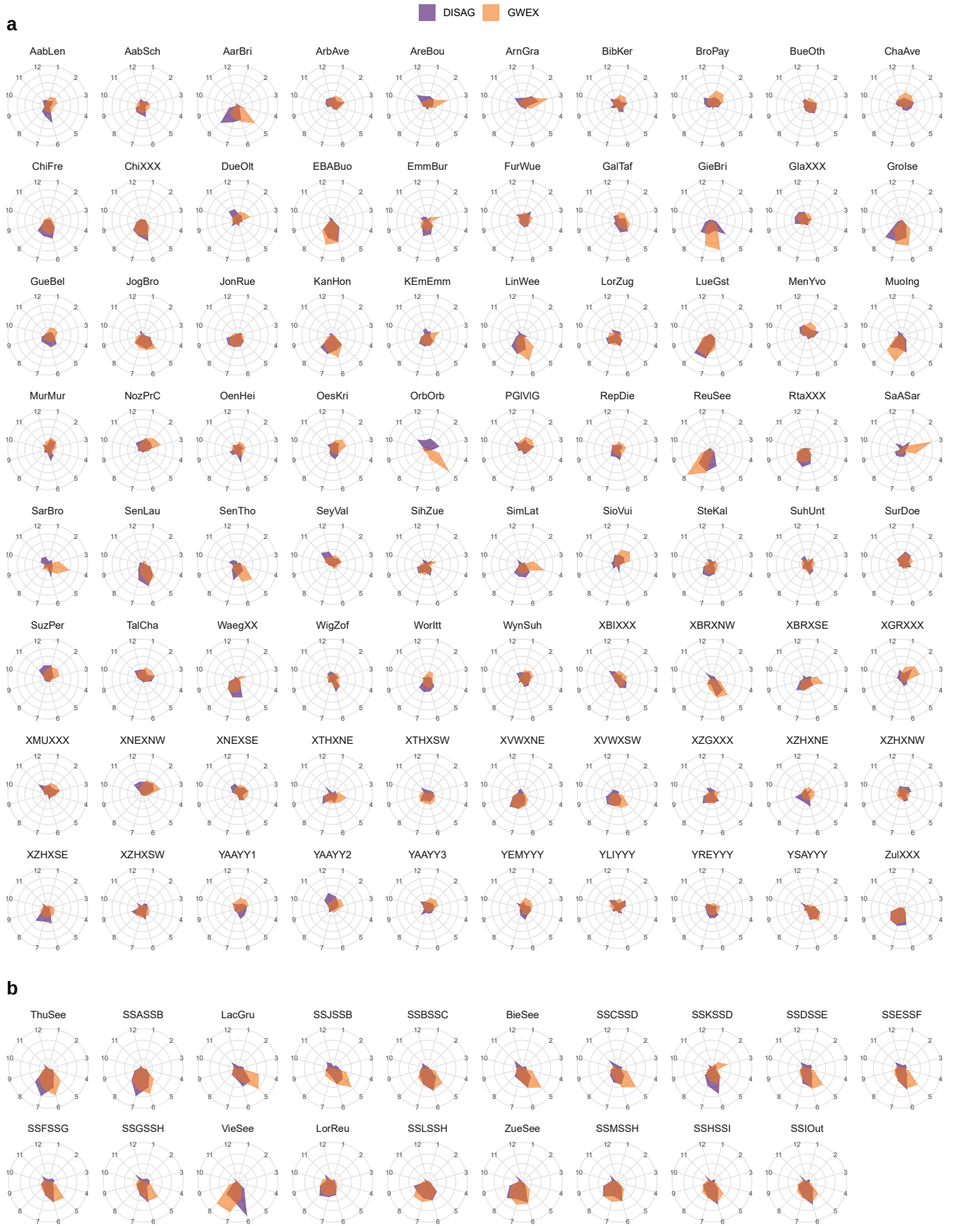
Figure S3. Seasonality of the largest annual 72-hour discharge events in simulations with disaggregated meteorology 1930–2014 (DISAG) and with GWEX scenarios. Panel a: 80 HBV sub-catchments; panel b: 19 RS MINERVE output nodes.
