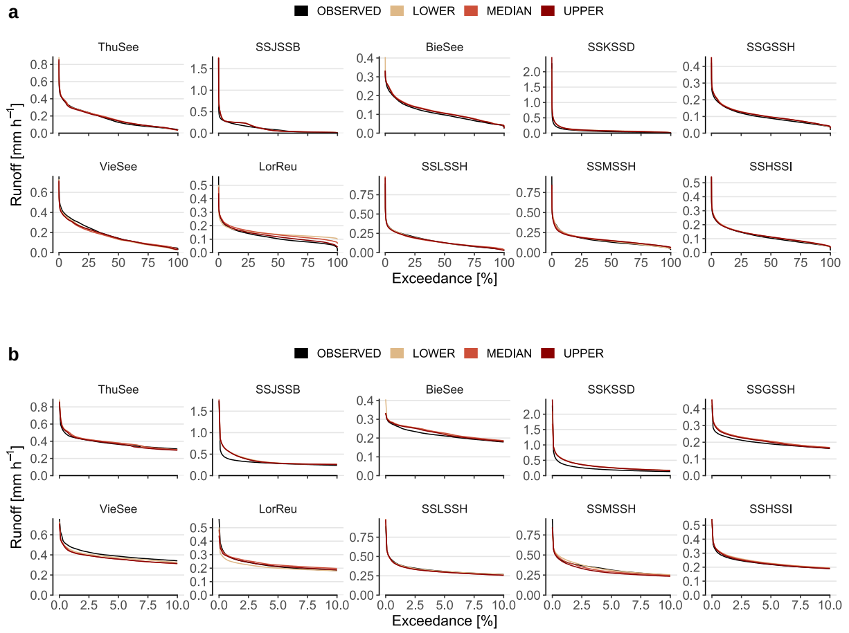
Figure S2. Panel a: Flow duration curves for 10 gauged output nodes of RS MINERVE (lower, median and upper representative parameter sets; time period 1930–2014; ordered by location along the Aare River) in comparison to observations (varying time periods, see Table S2). Panel b: Similar plots for highest 10% of flows.
