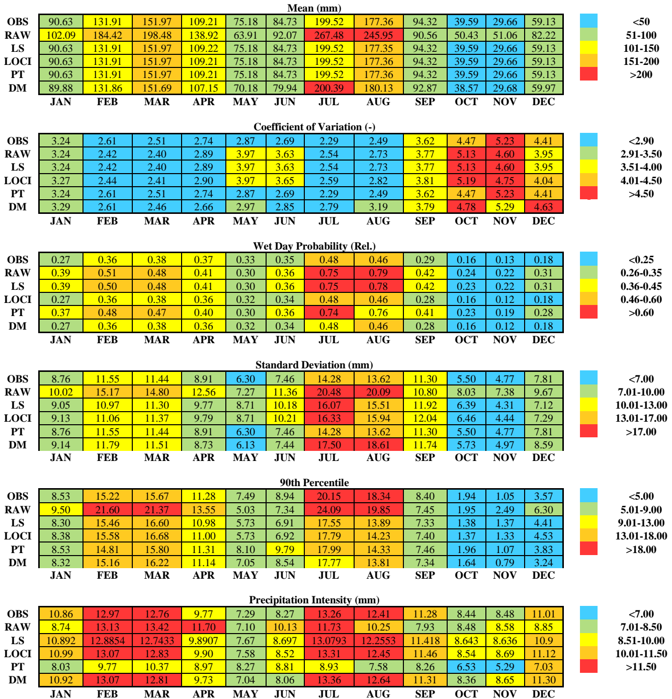
Figure S1: Comparison of raw and bias corrected ERA5 precipitation statistics against observed precipitation for the period 1981-2014
