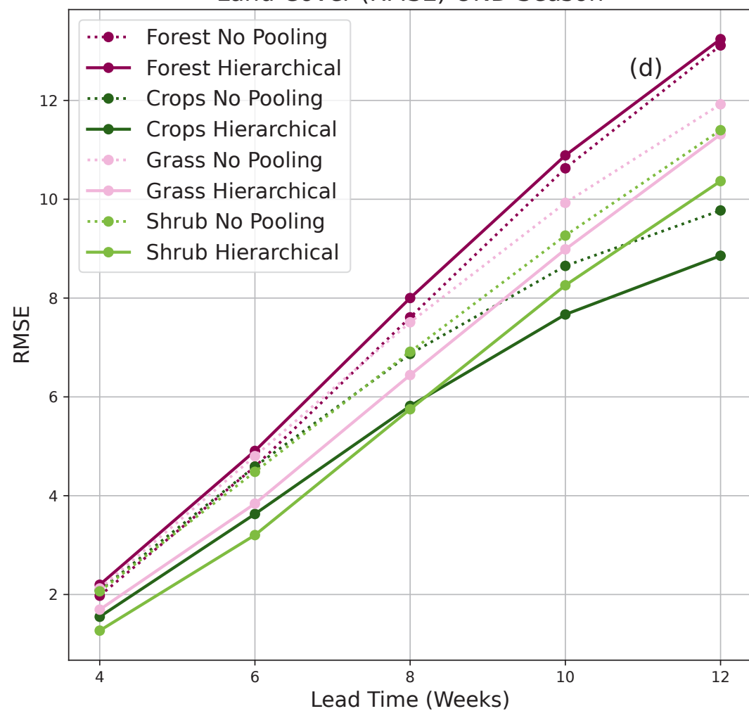
Land Cover (RMSE) OND Season
