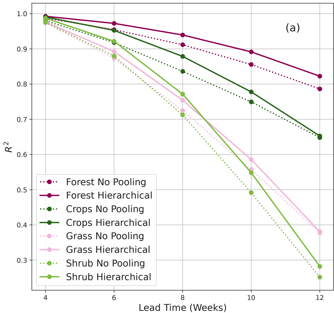
Land Cover R^2 OND Season
