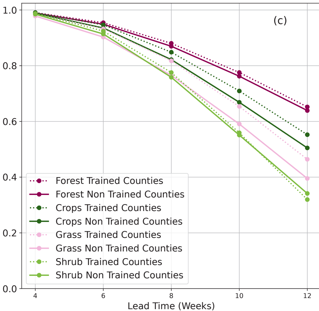
Land Covers R^2
