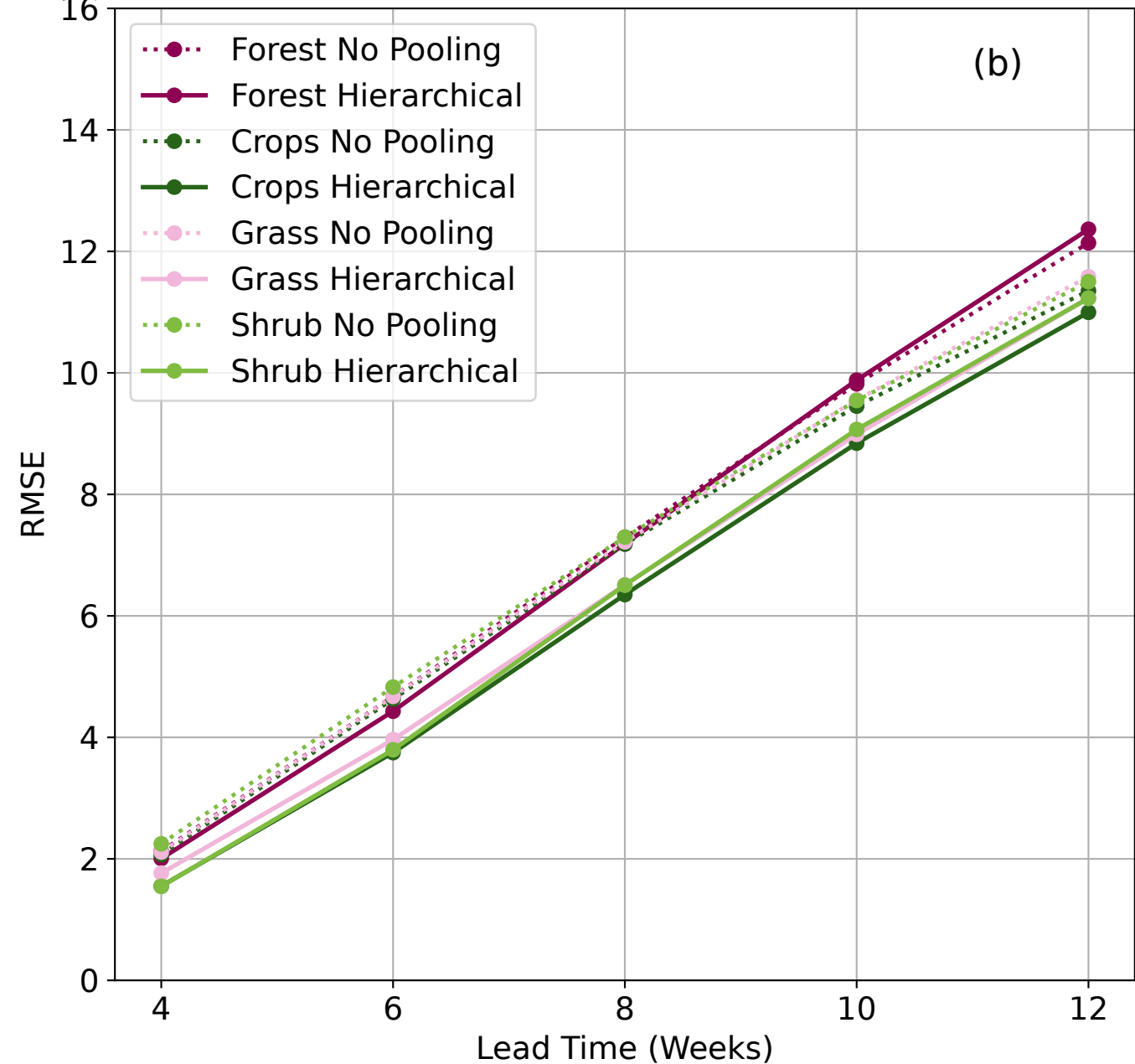
Land Cover (RMSE)
