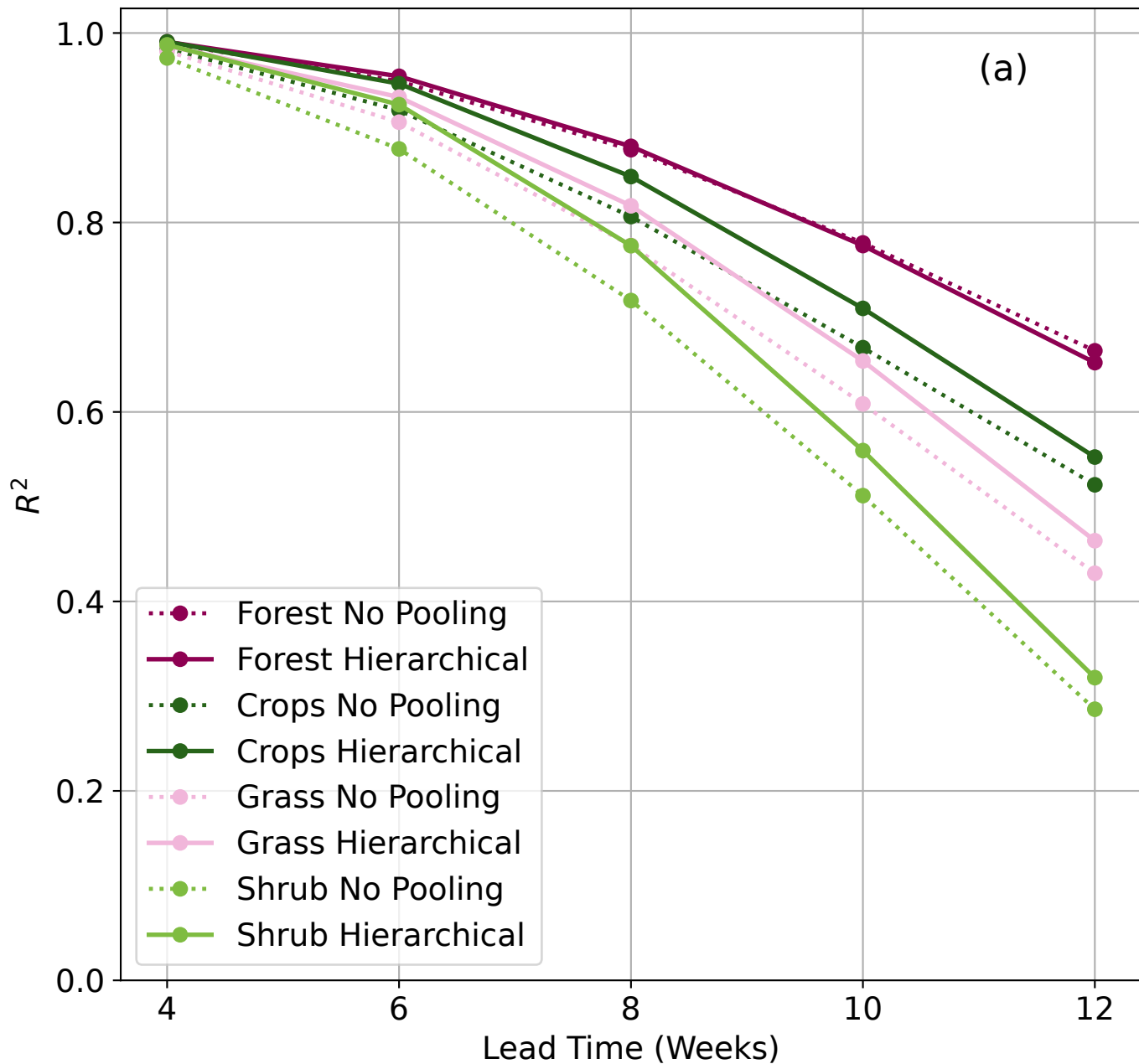
Land Cover R^2
