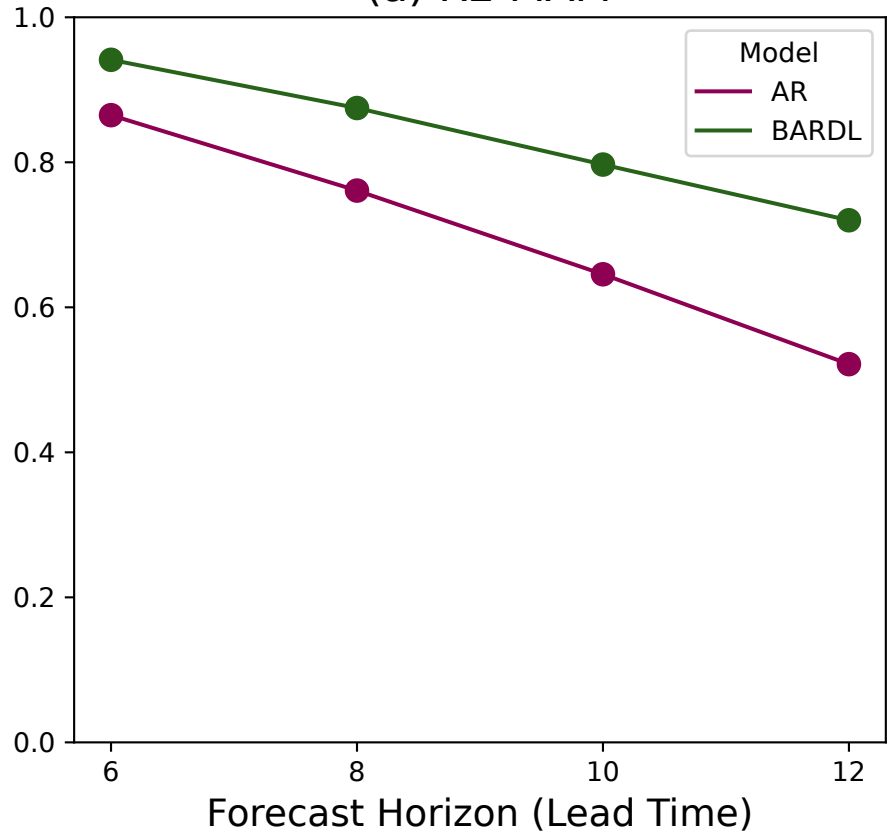
(c) R2 OND
