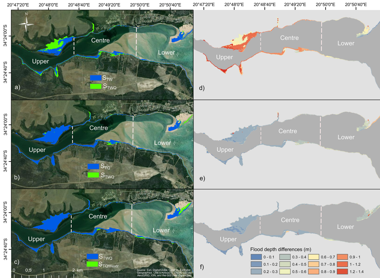
Figure 5. Comparison of flood extents of compound scenario and that excluding the driver (a–c) and differences in flood depths (d–f). Panel (d) shows the flood depths of S_{TWQ}-S_{TW} , (e) shows S_{TWQ}-S_{TQ} , and (f) shows S_{TWQextr}-S_{TWQ} .
