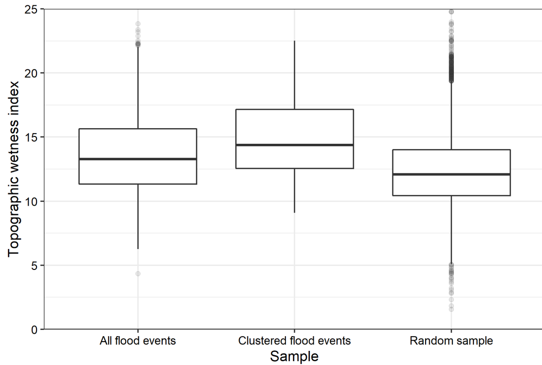
Figure S6: Topographic Wetness Index (TWI) for flood events in Quito recorded in Ecuador's Open Government Database. The TWI is shown for all flood events ( n = 1,274 ), clustered flood events where two events are recorded within 40 m of each other ( n = 125 ), and a random sample of TWI values ( n = 10,000 )
