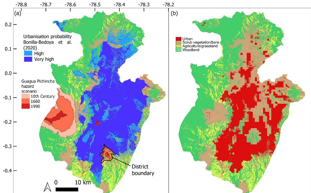
Figure S3. (a) Urbanisation probability from Bonilla-Bedoya et al. (2020). Guagua Pichincha Volcano hazards scenarios are shown from IG-EPN et al. (2019). (b) Modified Bonilla-Bedoya et al. (2020) scenario, which excludes urbanisation on the steep slopes of Guagua Pichincha Volcano and for category 5 (high) landslide susceptibility (Fig. S3) (Stanley and Kirschbaum, 2017). An urbanised area crossing the Metropolitan District Boundary was also included.
