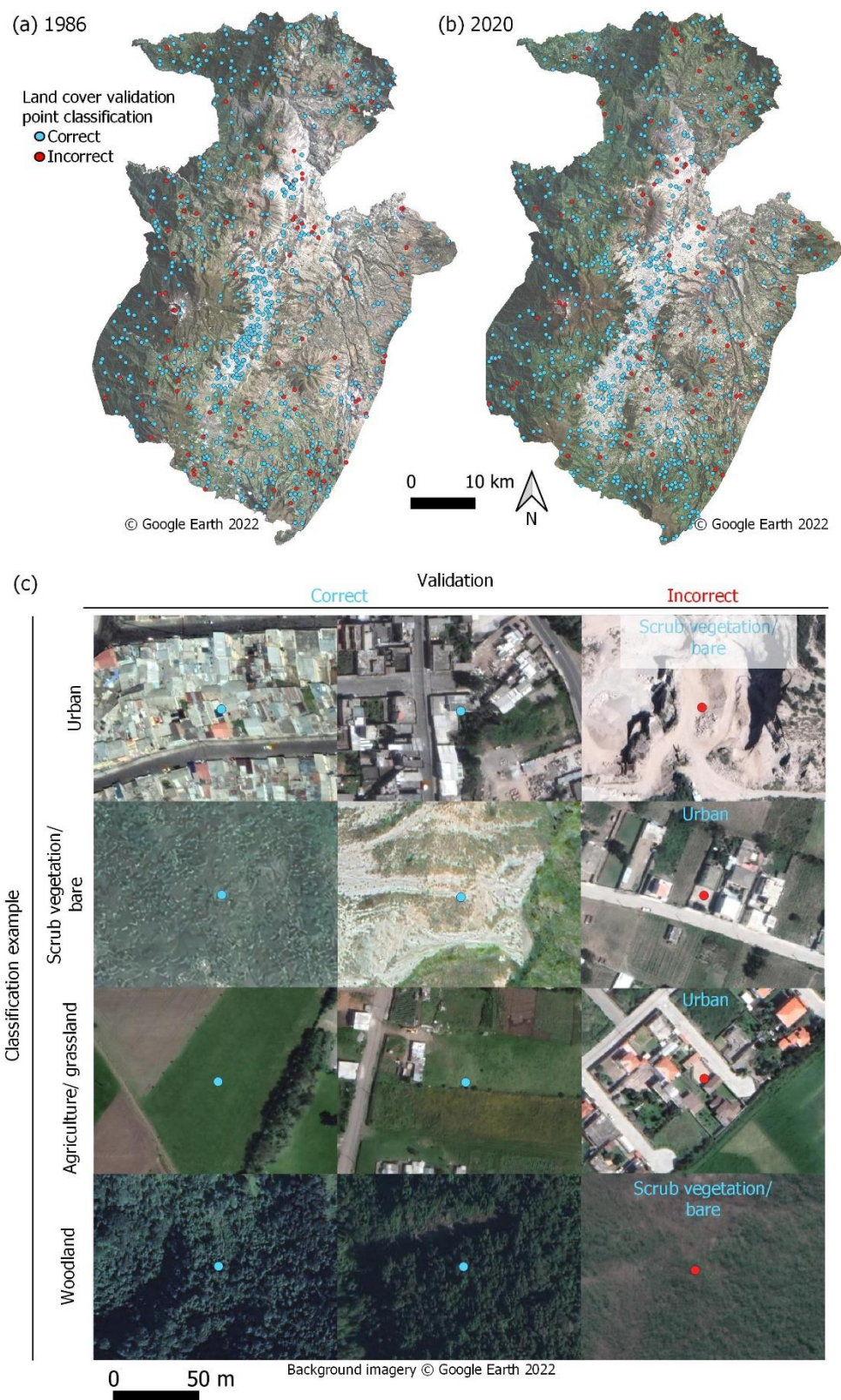
Figure S2. (a-b) Validation of the Random Forest Classification using 800 validation points. (c) Example land cover classifications and corresponding satellite imagery from a Google Earth basemap (© Google Earth).
