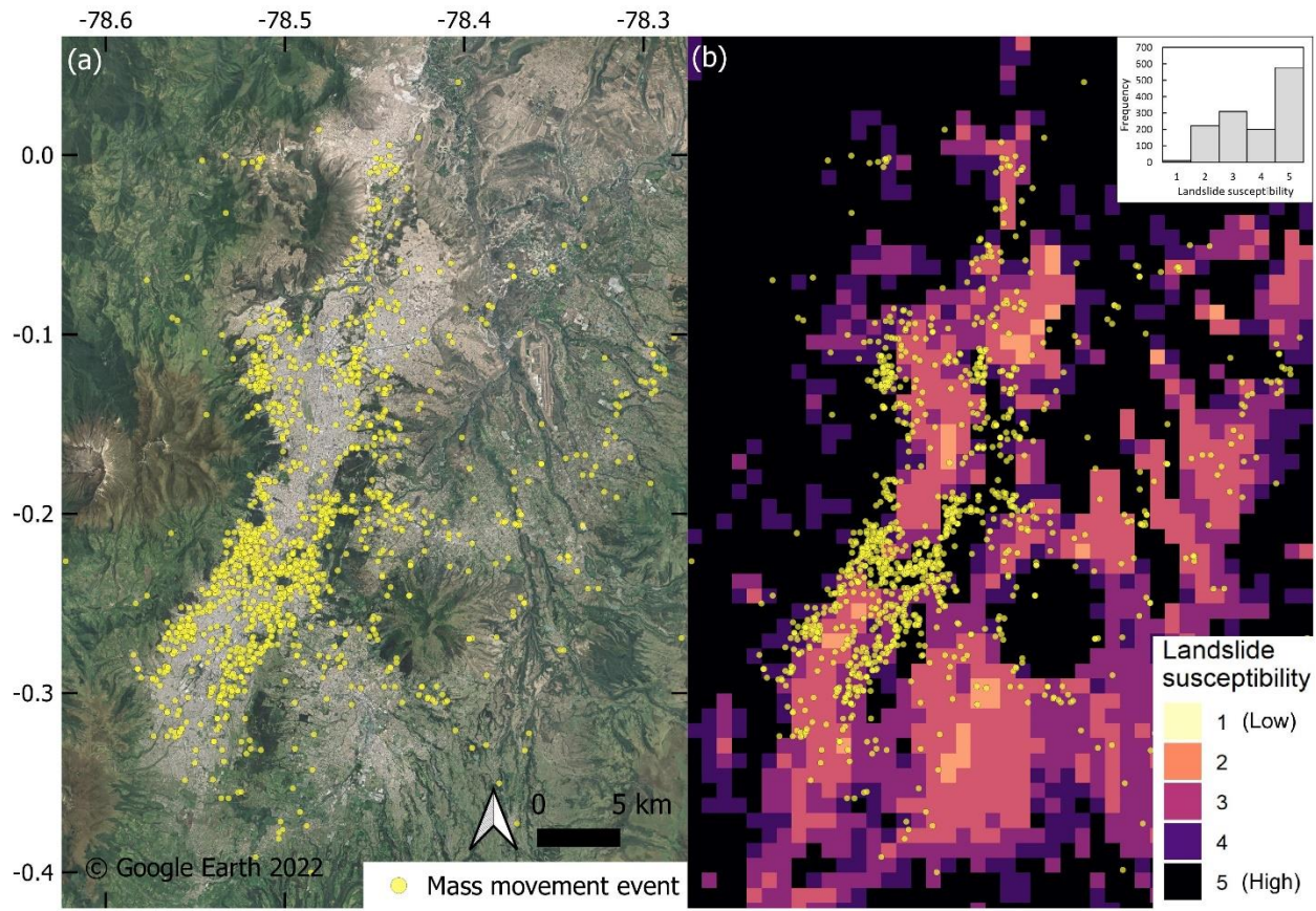
Figure S4: (a) Open Government records of movement events 2006–2017 ( n = 1321 ). (b) Spatial distribution of the recorded mass movement events in relation to the landslide susceptibility model (Stanley and Kirschbaum, 2017). Inset shows the frequency of events falling within each category.
