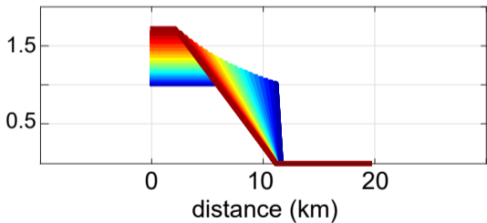
(b) coseismic slip (m)
