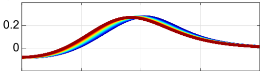
(a) surface deformation (m)
