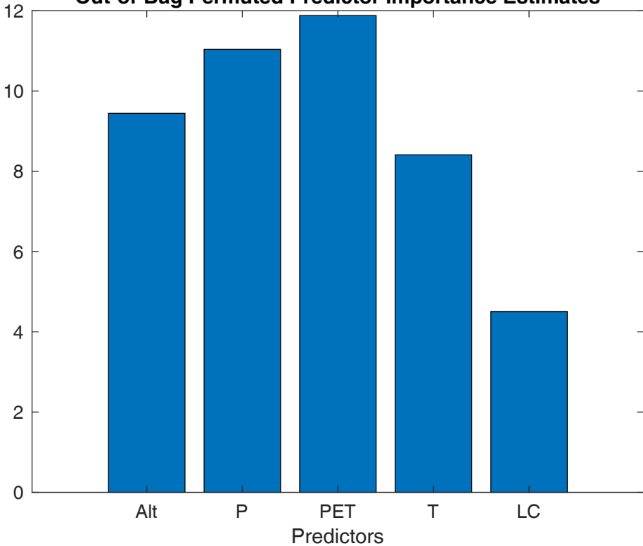
Out-of-Bag Permuted Predictor Importance Estimates
