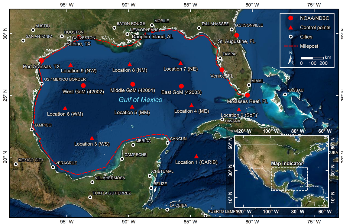
Figure 2. Area of interest of the Gulf of Mexico, including the locations of the nine control points in the GoM (red triangles), NOAA/NDBC measurement location (red dots), cities (white circles) and milepost (red dashed line). © Esri, DigitalGlobe, GeoEye, Earthstar Geographics, CNES/Airbus DS, USDA, USGS, AeroGRID, IGN and the GIS User Community. Sect. 3.2.
