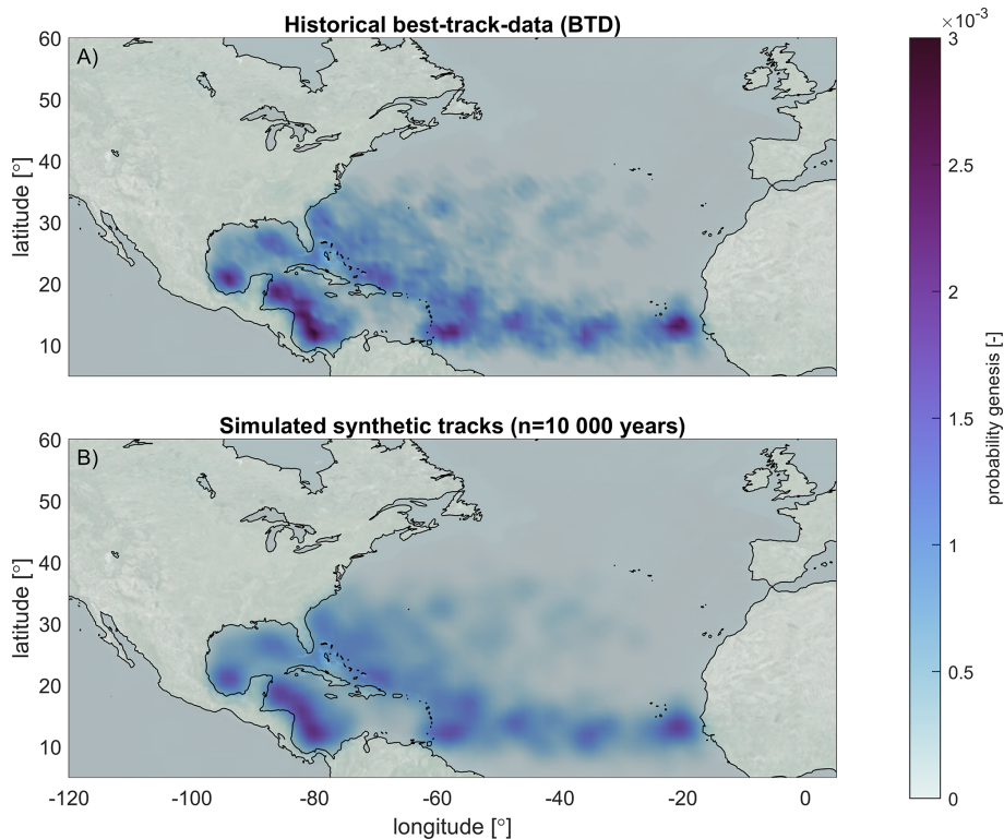
Figure 3. Genesis probability of historical BTD (a) and simulated TCs with TCWiSE (b) for the NA basin. Occurrence is based on TCs within 200 km per grid cell for historical TCs from 1886–2019 and 10 000 years of simulated events. © Microsoft Bing Maps.
