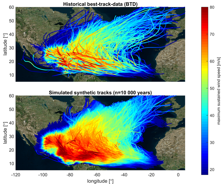
Figure 4. (a) Overview of historical tropical cyclone tracks in the IBTrACS database for the period 1886–2019. (b) 10 000 years of simulated tracks with TCWiSE. Colors indicate the maximum intensity of the eye. Note that the maximum intensity is the maximum wind speed at the core of the TC, which is different from the temporally and spatially varying wind field and/or spatially varying wind swaths. In particular, further away from the TC eye, gale-force winds can still be present due to the TC. © Microsoft Bing Maps.
