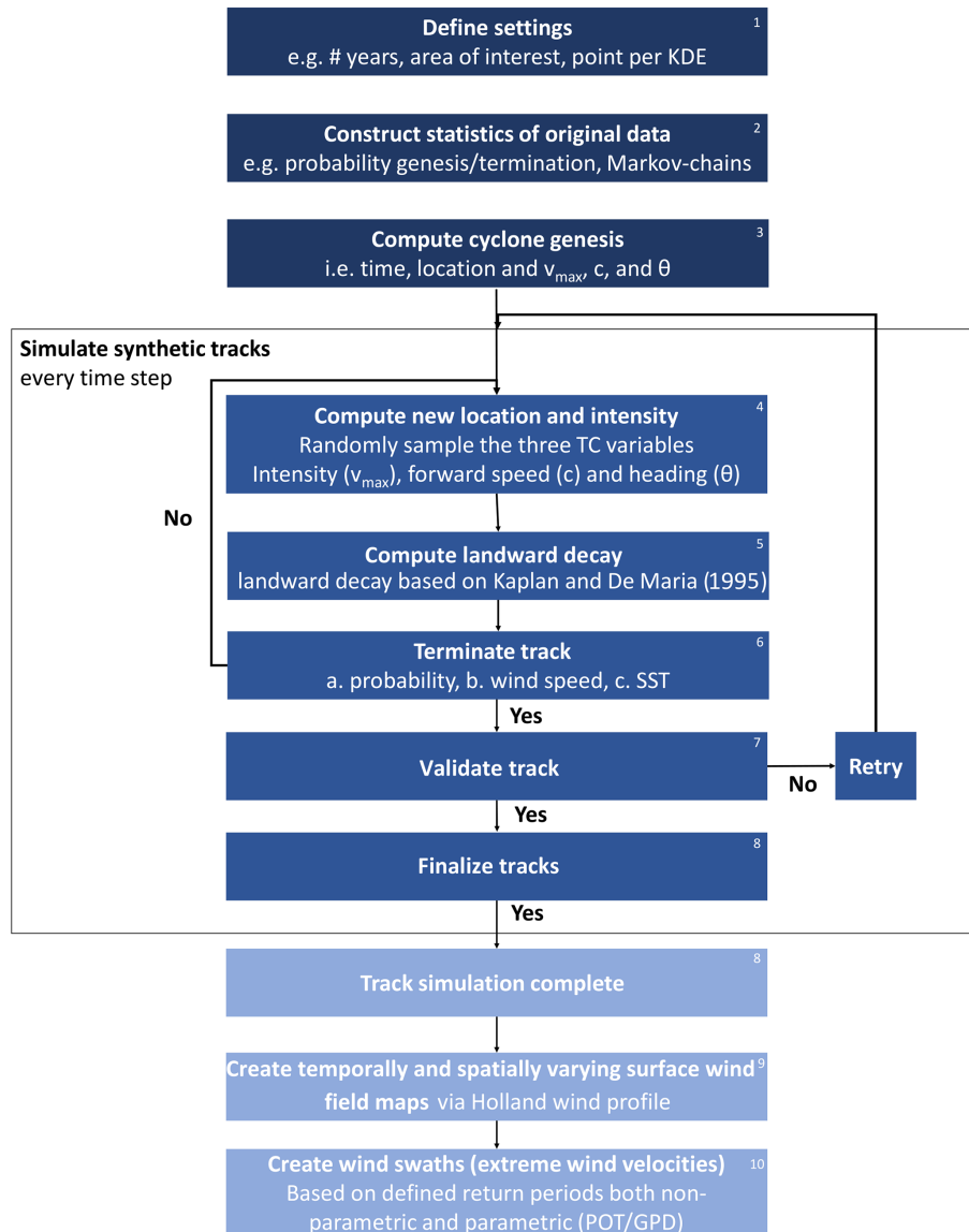
Figure 1. Flowchart of the track modeling procedure. Dark blue colors are pre-processing steps, blue colors the computational core of TCWiSE and light blue post-processing steps. KDE stands for kernel density estimation, SST stands for sea surface temperature and POT/GPD is the acronym of peak over threshold and generalized Pareto distribution.
