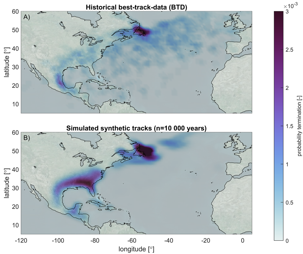
Figure 9. Termination probability of historical BTD (a) and simulated TCs with TCWiSE (b) for the NA basin. Occurrence is based on TCs within 200 km per grid cell for historical TCs from 1886–2019 and 10 000 years of simulated events. © Microsoft Bing Maps.
