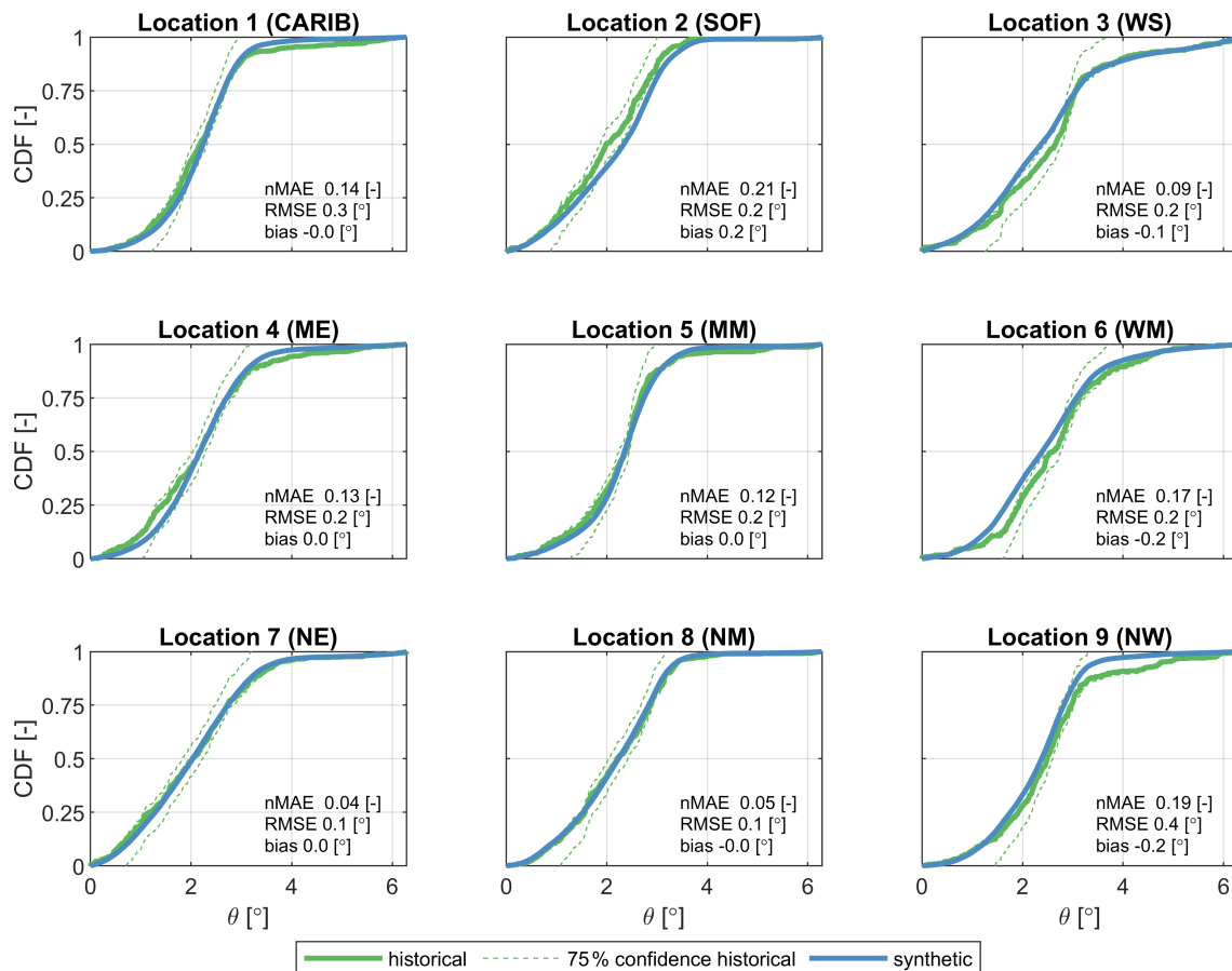
Figure 7. CDFs of heading ( \theta [°]) of historical (green line) and synthetic (blue line) TCs at 9 locations within the NA basin, as shown on the map in Fig. 2. The 75 % confidence interval (dashed green line) of historical data is also shown. Historic data are based on data available between 1886 and 2019, while synthetic data are derived from 10 000 years of simulated events with TCWiSE. Data points within 200 km from the control location are included in the analysis for both the historical and synthetic data.
