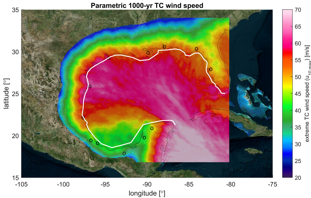
Figure 12. Model estimates for the parametric empirical estimate of 1000-year TC wind speed return values based on extreme wind speeds based on 10 000 years of TCWiSE computations. All wind speeds are in meters per second, 10 min averaged and determined at a 10 m height. Black dots are the location of cities as plotted in Figs. 10 and 13. © Microsoft Bing Maps.
