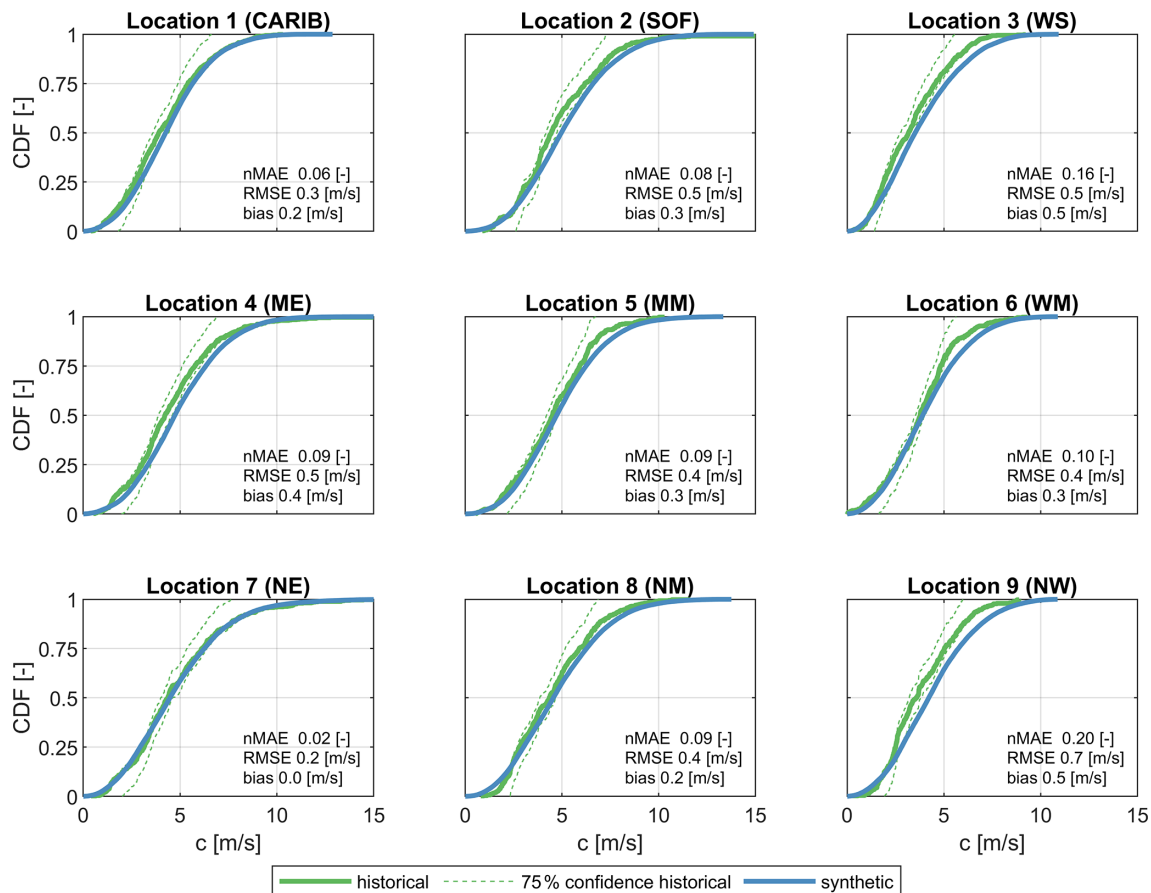
Figure 6. CDFs of forward speed ( c [ \text{m s}^{-1} ]) of historical (green line) and synthetic (blue line) TCs at nine locations within the NA basin, as shown on the map in Fig. 2. The 75 % confidence interval (dashed green line) of historical data is also shown. Historic data are based on data available between 1886 and 2019, while synthetic data are derived from 10 000 years of simulated events with TCWiSE. Data points within 200 km from the control location are included in the analysis for both the historical and synthetic data.
