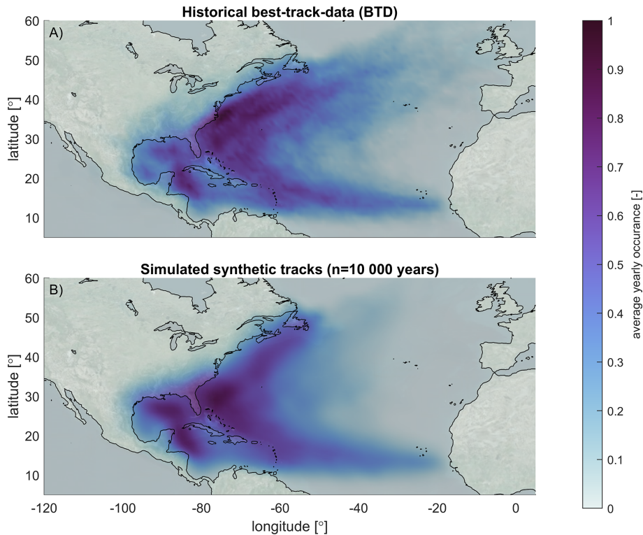
Figure 5. Average occurrence of historical BTD (a) and simulated TCs with TCWiSE (b) for the NA basin. Occurrence is based on TCs within 200 km per grid cell for historical TCs from 1886–2019 and 10 000 years of simulated events. © Microsoft Bing Maps.
