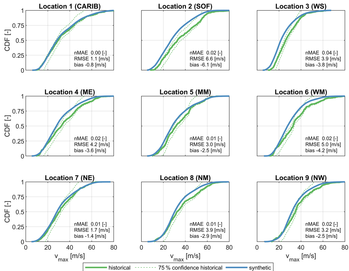
Figure 8. CDFs of maximum sustained wind speed ( v_{\max} [ \text{m s}^{-1} ]) of historical (green line) and synthetic (blue line) TCs at nine locations within the NA basin, as shown on the map in Fig. 2. The 75 % confidence interval (dashed green line) of historical data is also shown. Historic data are based on data available between 1886 and 2019, while synthetic data are derived from 10 000 years of simulated events with TCWiSE. Data points within 200 km from the control location are included in the analysis for both the historical and synthetic data.
