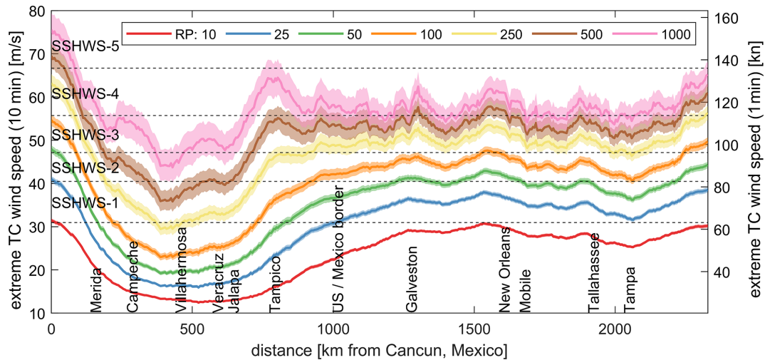
Figure 13. TCWiSE 10-, 25-, 50-, 100-, 250-, 500- and 1000-year return value estimates of wind speed. All wind speeds are in meters per second, 10 min averaged and determined at a 10 m height (left axis) or 1 min averaged in knots (right axis). Cities on the x axis are also depicted in Fig. 12 as black circles. Milepost is presented in the same figure as a white line. Shading shows the 5–95 % confidence interval. SSHWS value indicates the corresponding Saffir–Simpson hurricane wind scale.
