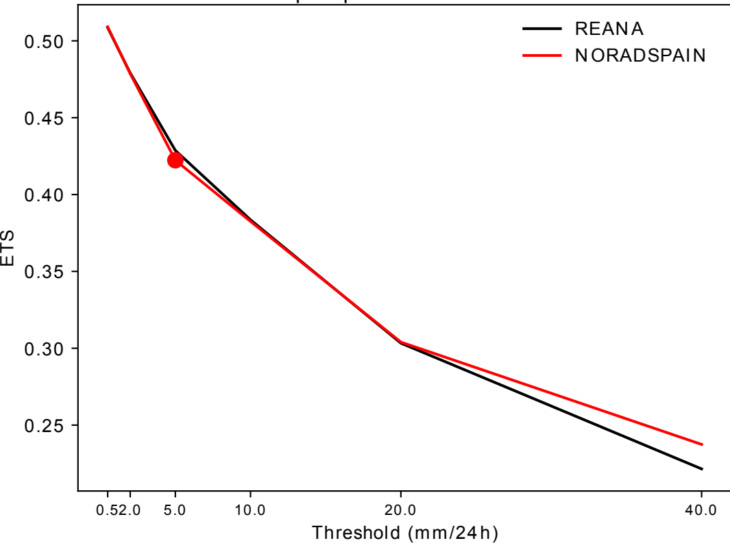
24 h accumulated precipitation between 30 and 54 h
