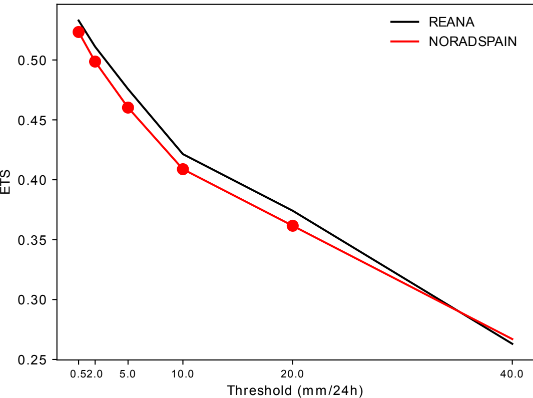
24 h accumulated precipitation between 6 and 30 h
