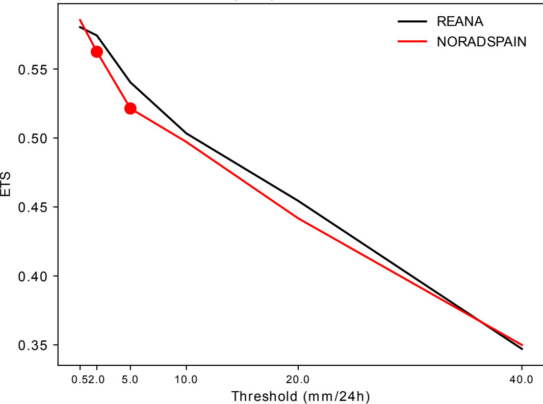
24 h accumulated precipitation from the 3 h forecasts
