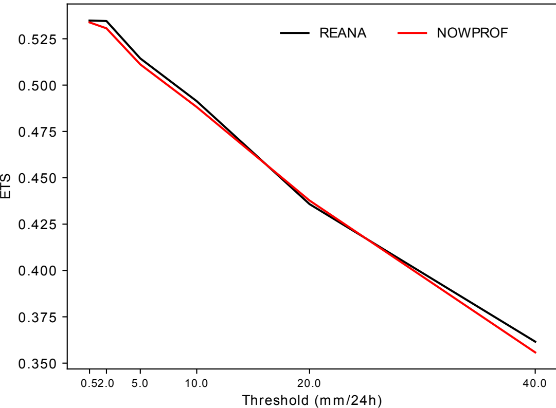
24 h accumulated precipitation between 6 to 30 h
