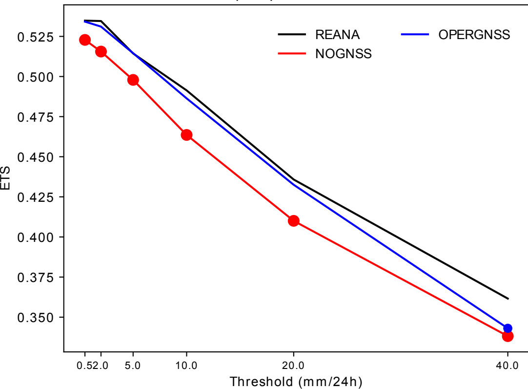
24 h accumulated precipitation from the 3h forecasts
