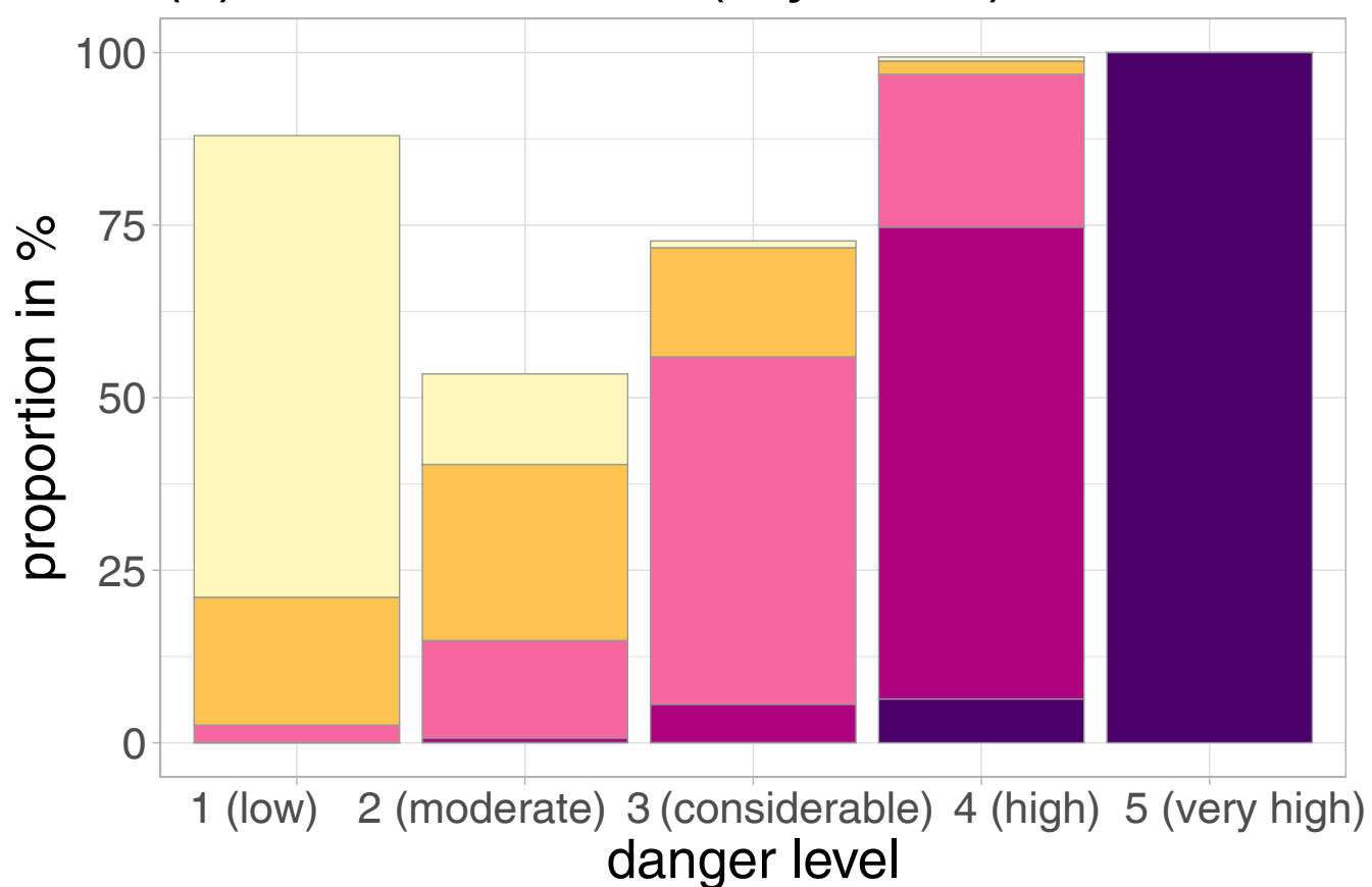
(e) avalanche size (dry snow)
