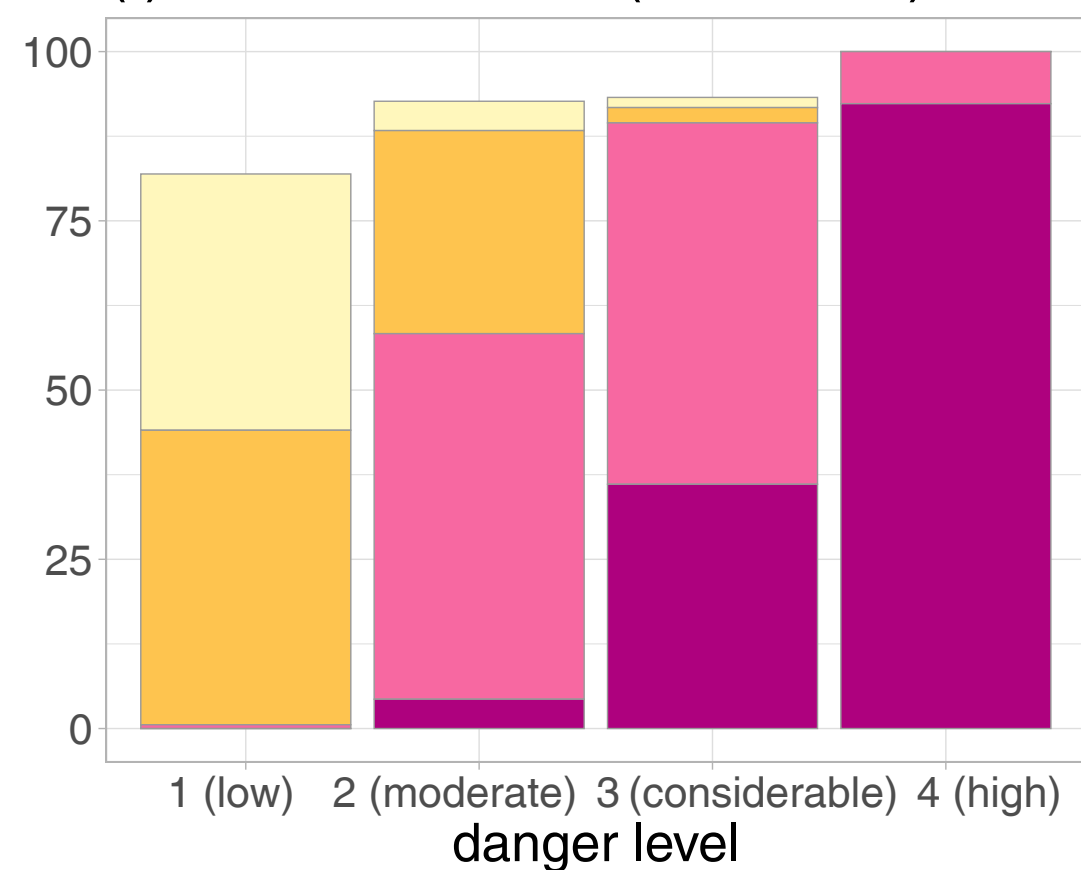
(f) avalanche size (wet snow)
