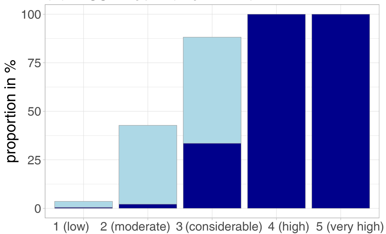
(a) trigger type (dry snow)
