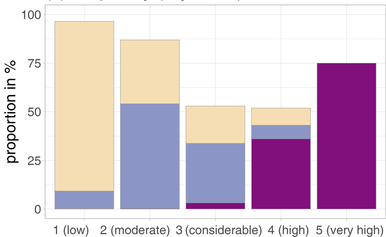
(c) frequency (dry snow)
