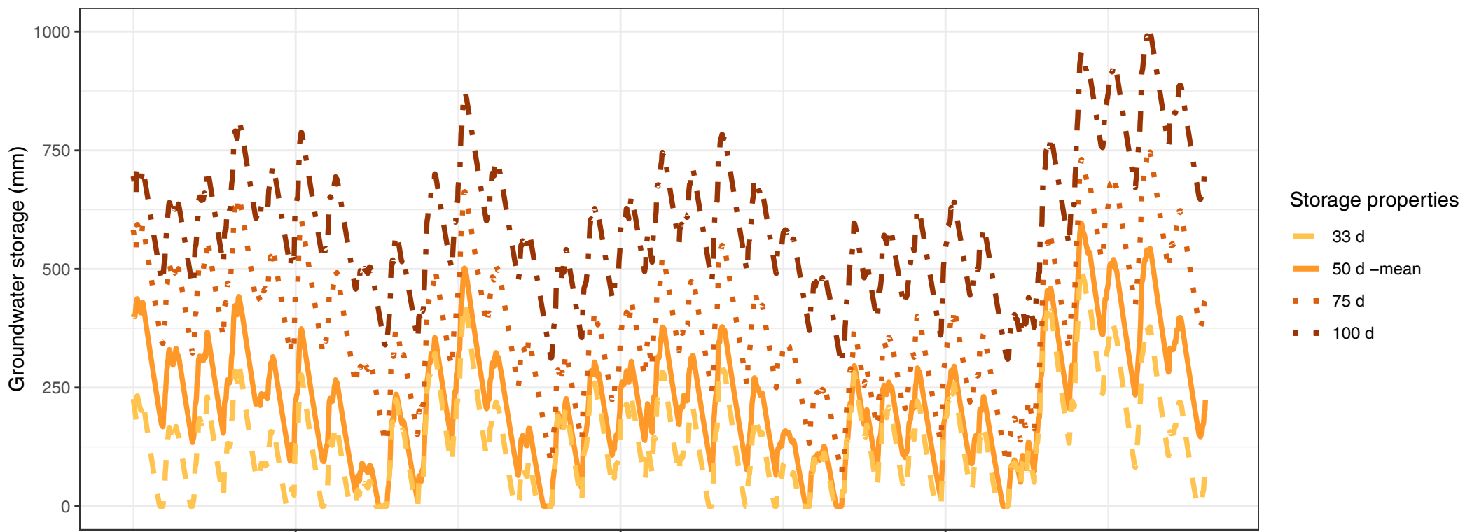
(a) Large groundwater storage system
