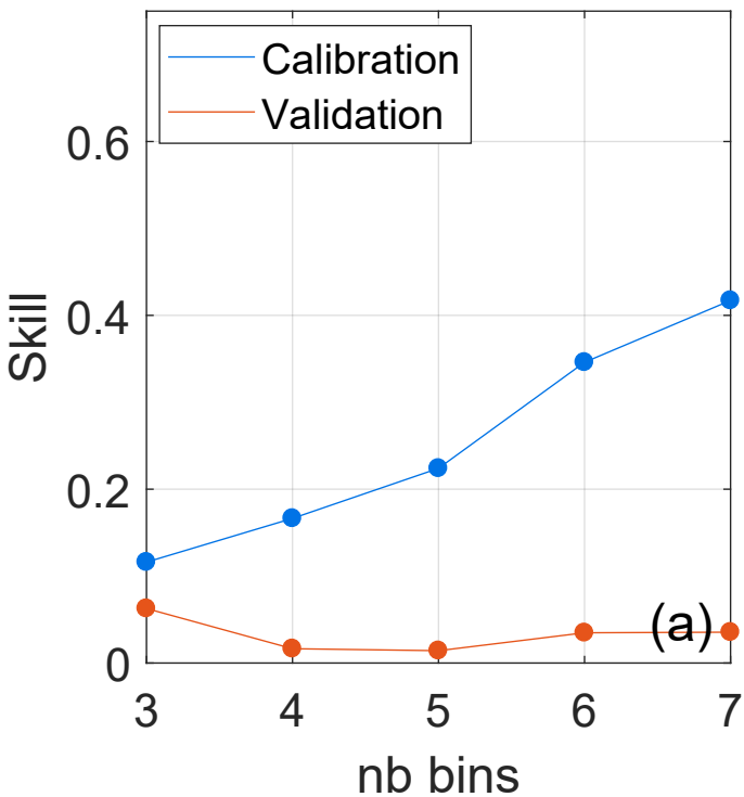
Skill
