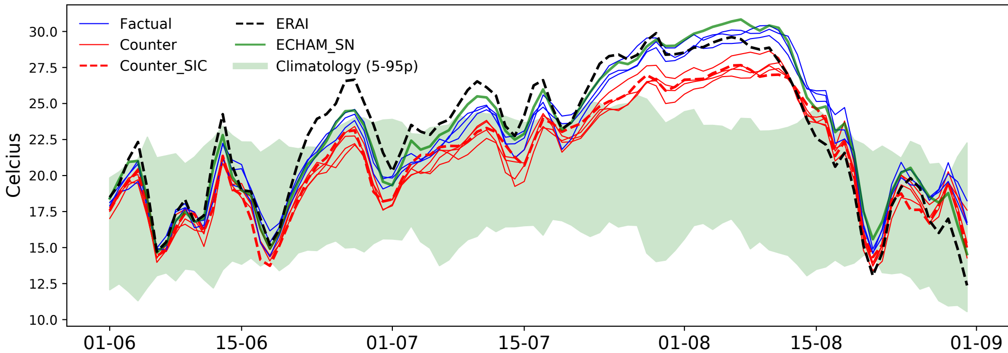
(b) Russian Heatwave 2010
