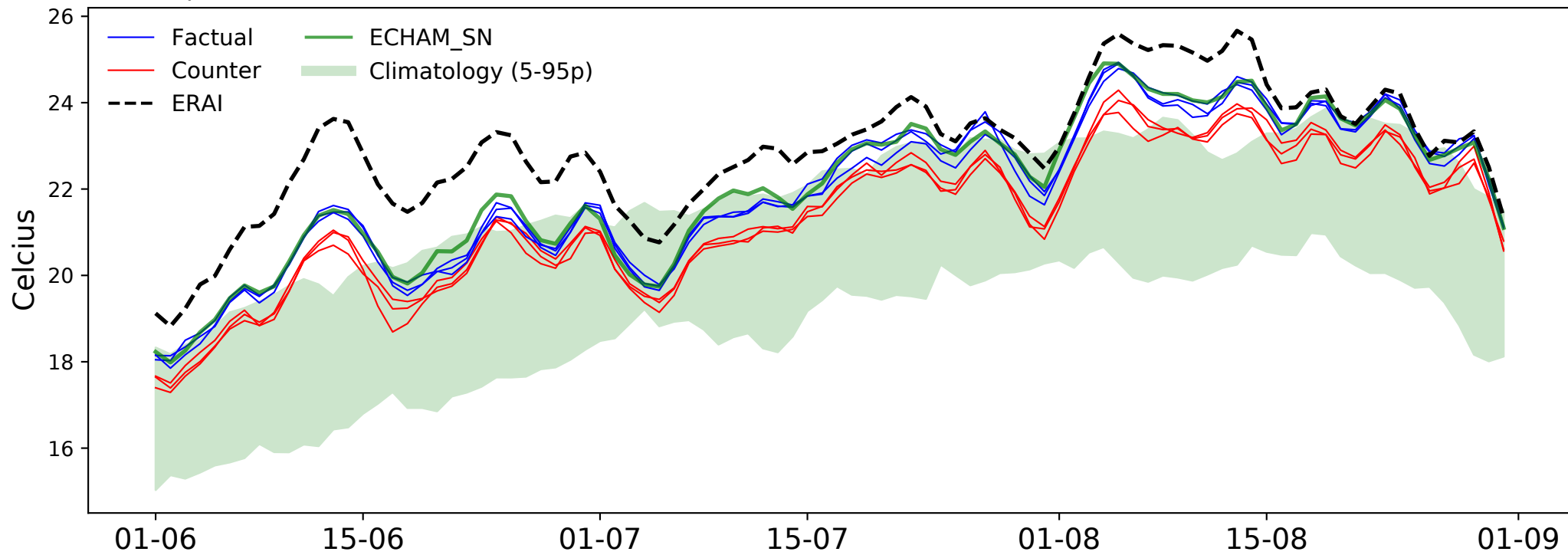
(a) European Heatwave 2003
