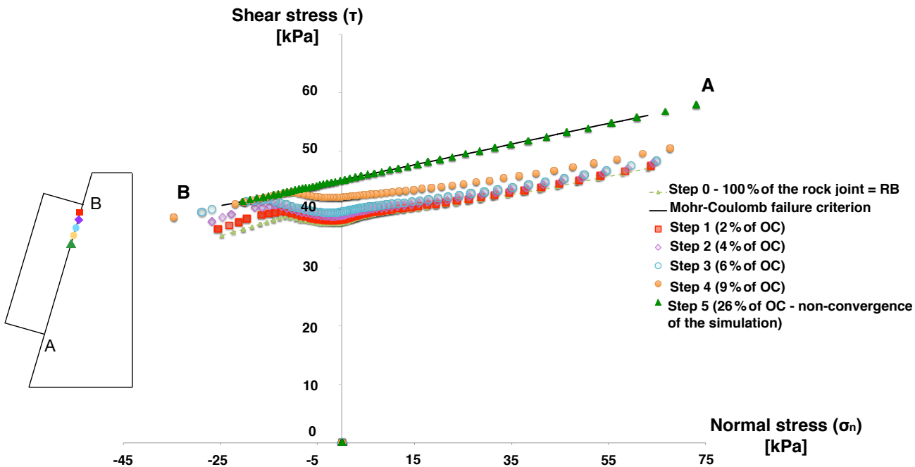
(b) Model 4 with rock bridges that failed (RBF) considered open crack (OC)
