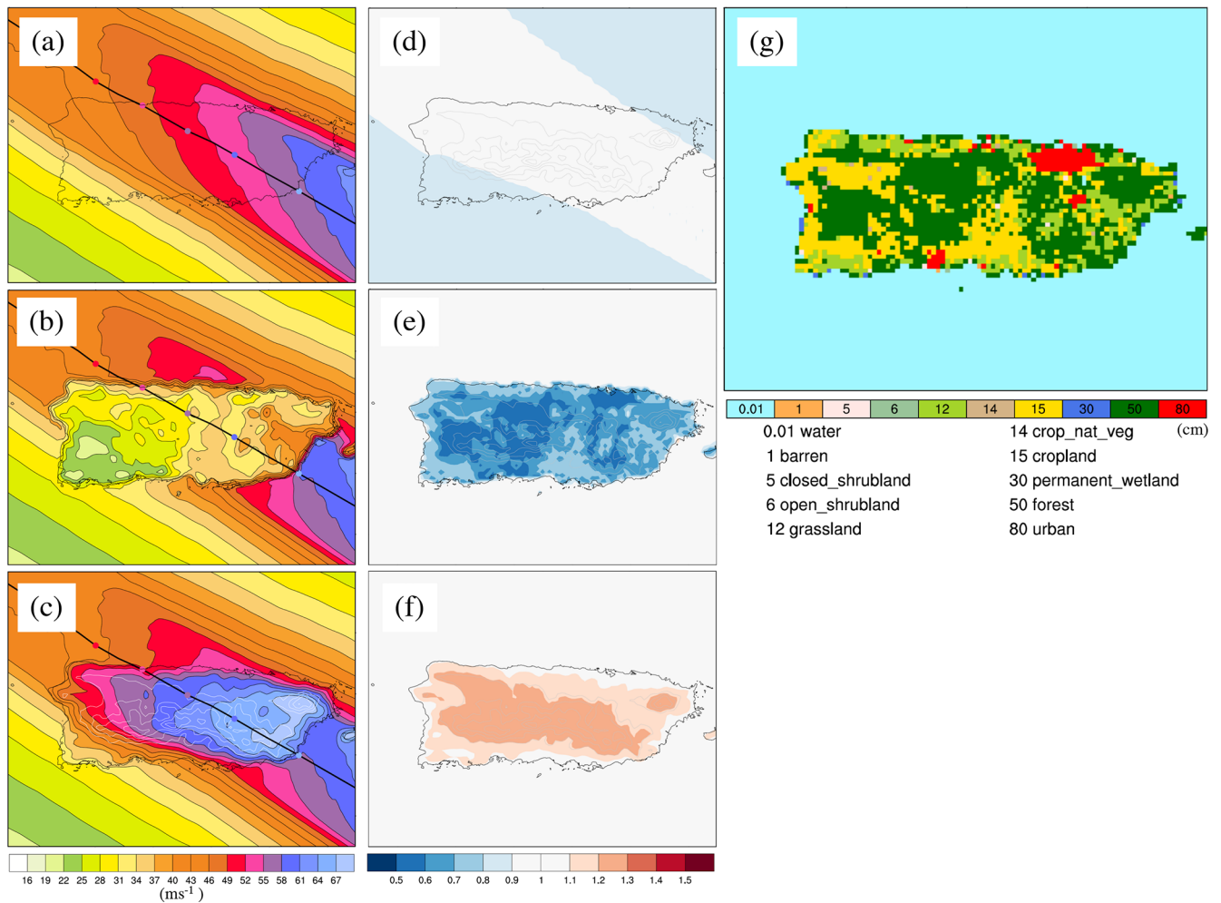
Figure 3. (a–c) Simulated footprints ( \text{ms}^{-1} ) of Hurricane Maria (2017) over Puerto Rico using Willoughby and KW01 with (a) no land (NO_LAND), (b) no terrain height (NO_OROG) and (c) constant surface roughness equal to the ocean value (NO_ROUGHNESS). The hurricane track is shown by the thick black line with input V_{\text{max}} shown every 6 h along the track (coloured dots). Coastlines are shown by the thin black lines and are only included in (a) to aid interpretation. (d) Ratio of Willoughby only to NO_LAND. (e) Ratio of NO_LAND to NO_OROG. (f) Ratio of NO_LAND to NO_ROUGHNESS. (g) Surface roughness (cm) of the land use categories.
