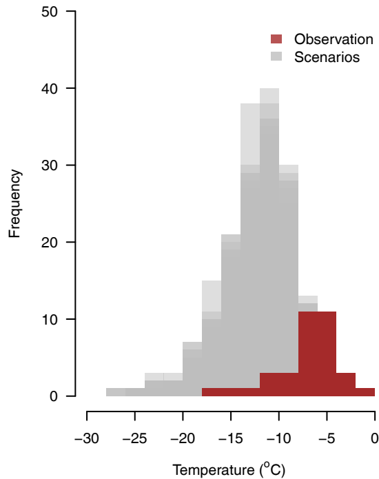
Annual min. daily temperature
