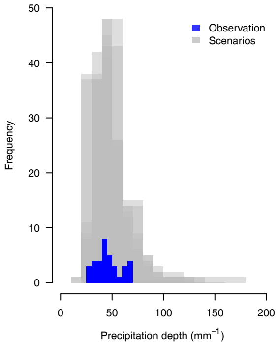
Annual max. daily precipitation depth
