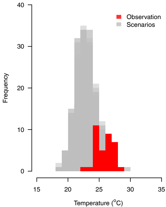
Annual max. daily temperature
