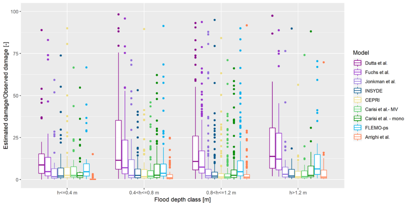
Figure S1: Estimated to observed damage ratios for different flood depth classes
