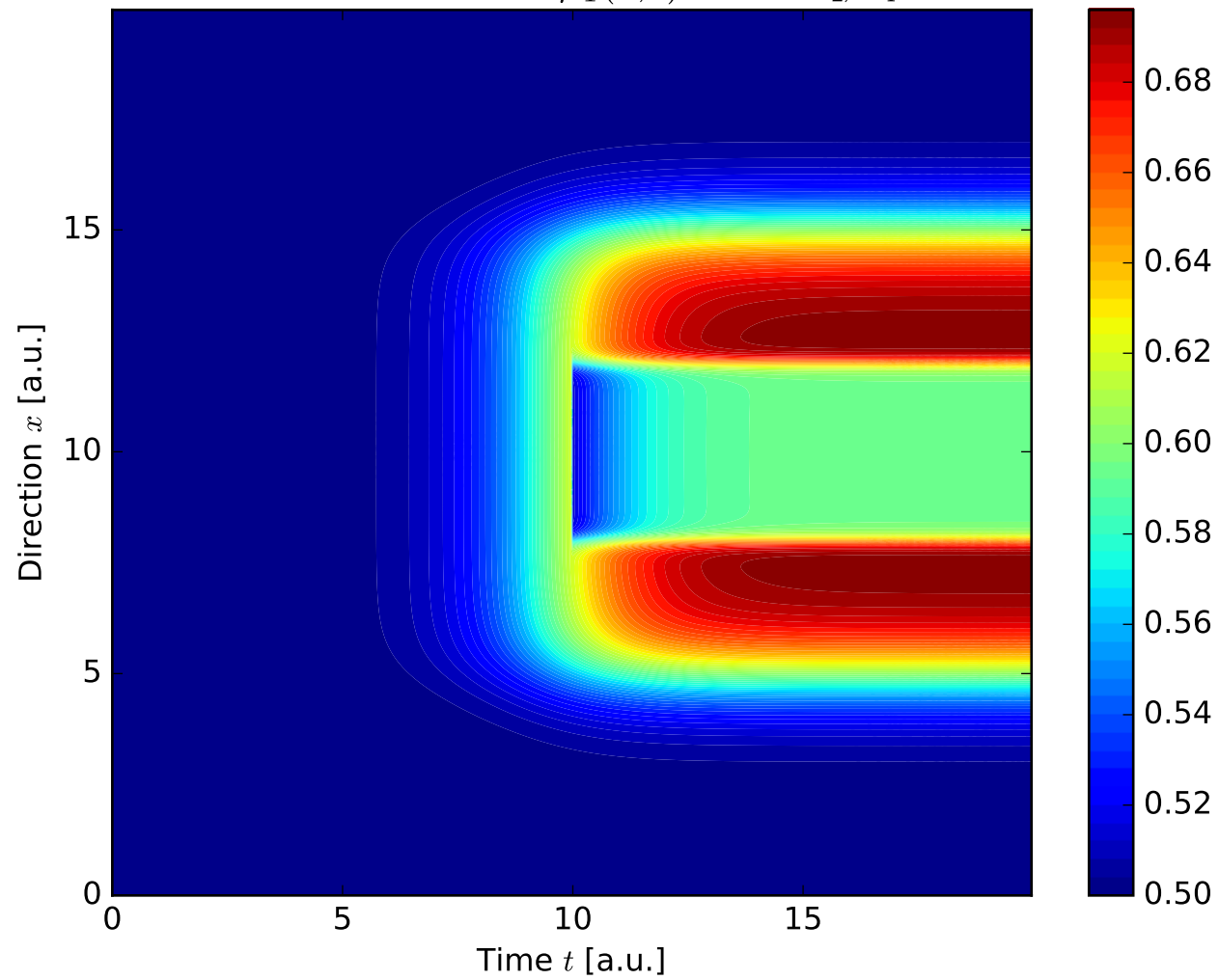
Total friction coefficient \bar{\mu}_T(x, t) . Case k_2, k_4 = 10^{-10}
