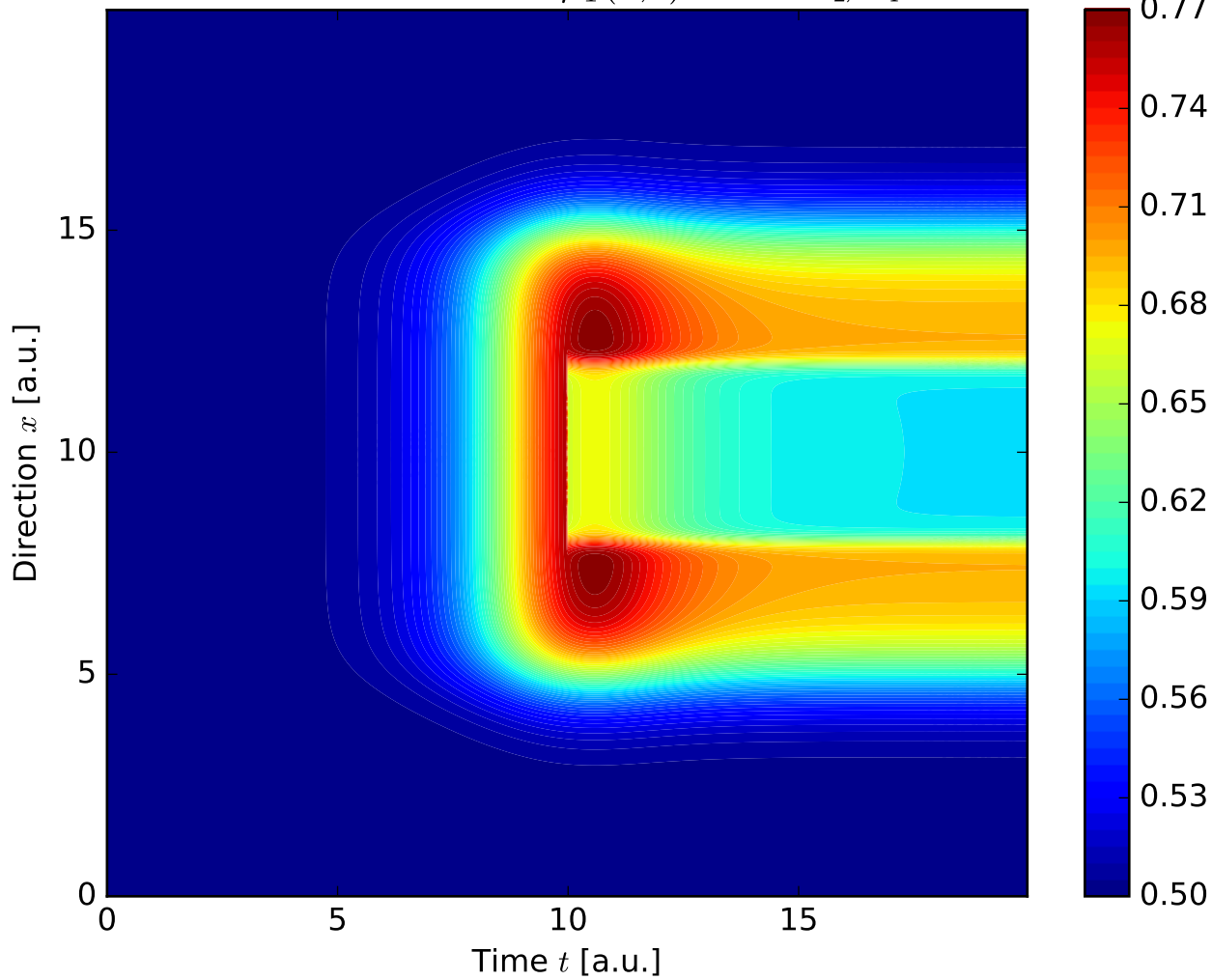
Total friction coefficient \bar{\mu}_T(x, t) . Case k_2, k_4 = 10^{-9}
