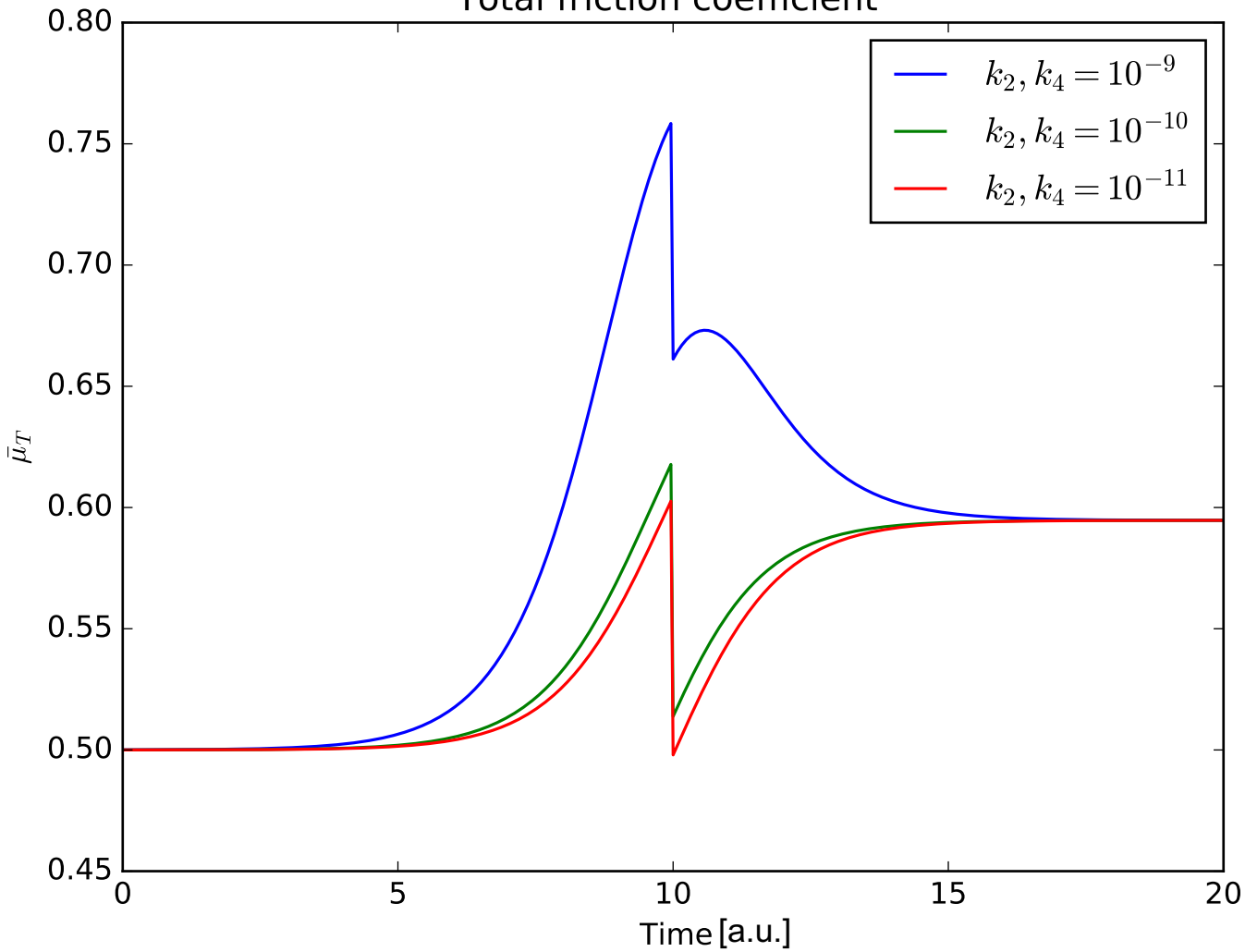
Total friction coefficient
