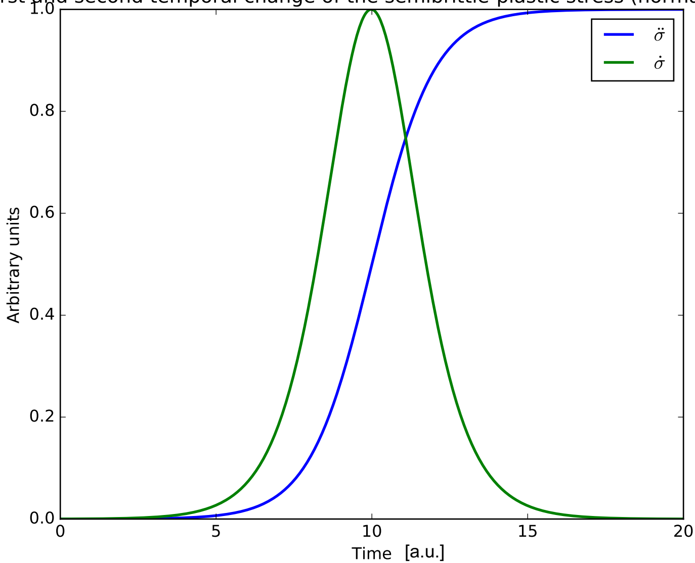
First and second temporal change of the semibrittle-plastic stress (normalized)
