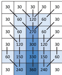
(c) Upslope contributing area [m 2 m -1 ]
