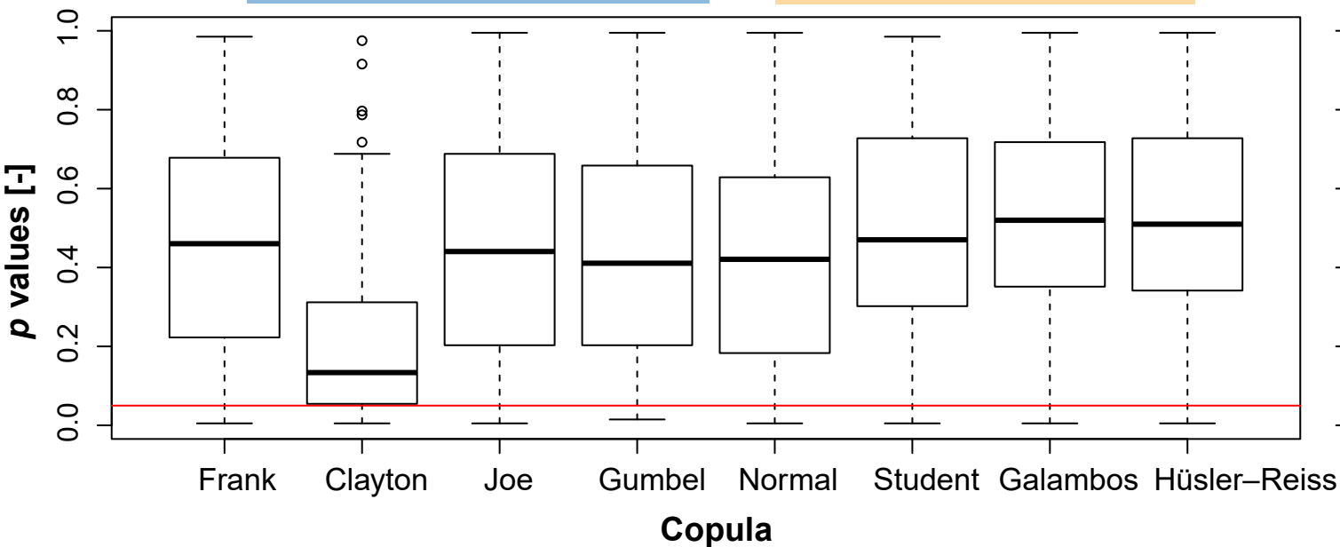
(c) Precipitation deficit duration and discharge deficit duration
