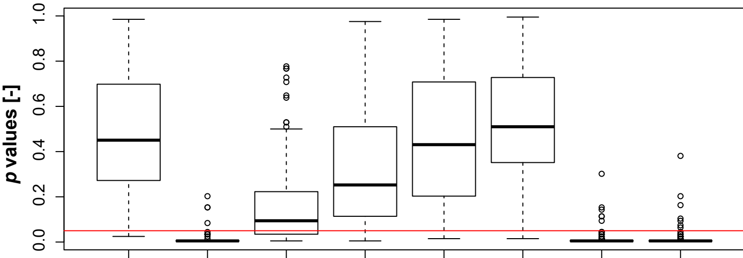
(c) Precipitation deficit duration and discharge deficit duration
