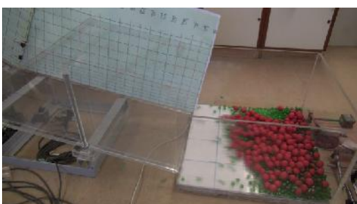
(a) Flow pattern of multi-size balls in physical test
