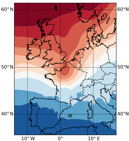
(c) 12 h forecast with D1 method
