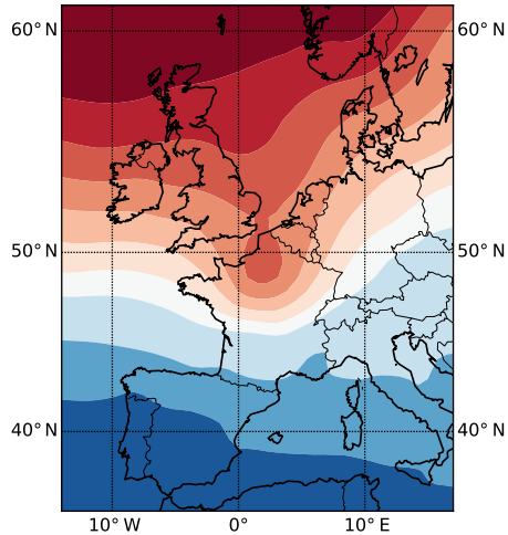
(b) ERA-Interim reanalysis
