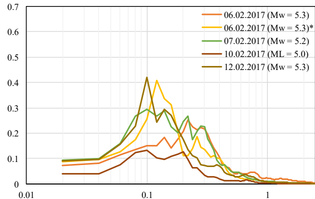
Elastic spectrum N-S ( \xi = \% 5 )
