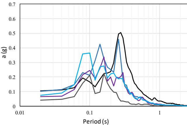
Elastic spectrum N-S ( \xi = \% 2 )
