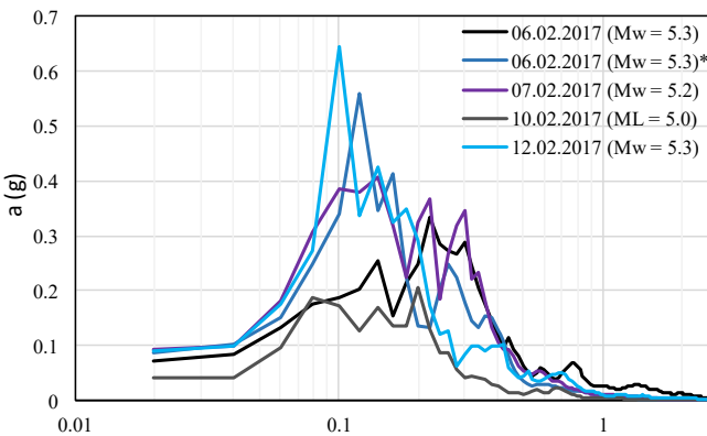
Elastic spectrum N-S ( \xi = \% 2 )
