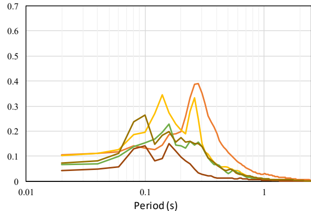
Elastic spectrum N-S ( \xi = \% 5 )
